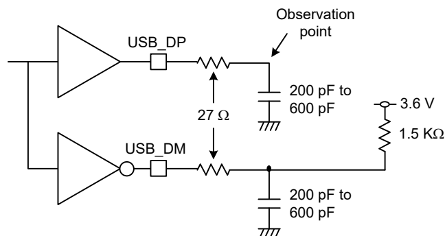
Figure 53.75 Test circuit in low-speed mode
