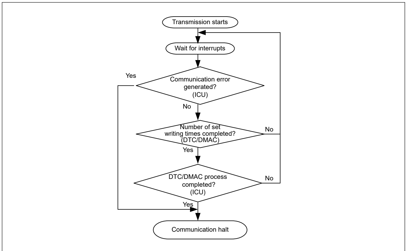
Figure 38.54 Transmission procedure
