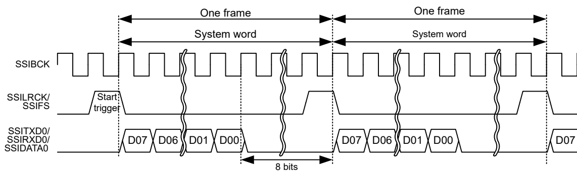
Figure 38.39 Short frame in monaural format (with padding: system word length > data word length)
