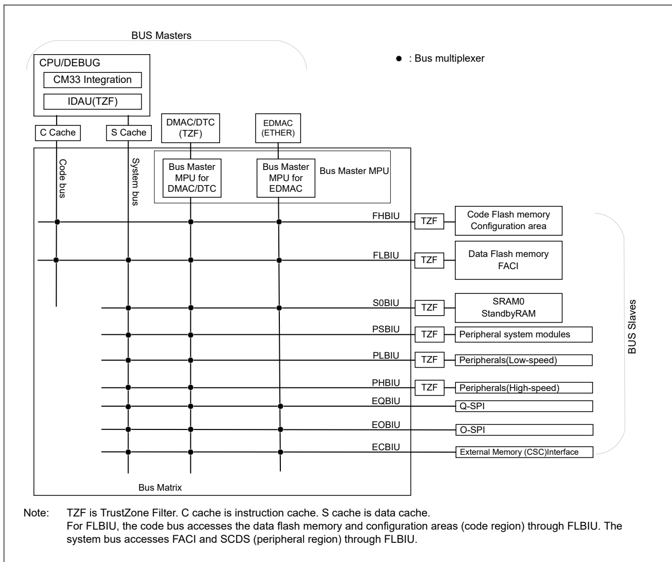
Figure 14.1 Bus Connection
