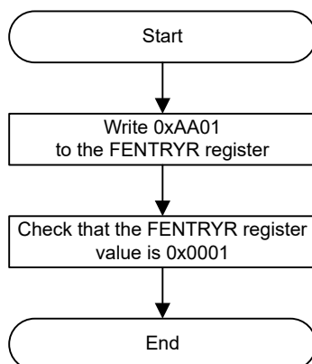
Figure 50.10 Procedure to transition to code flash P/E mode
