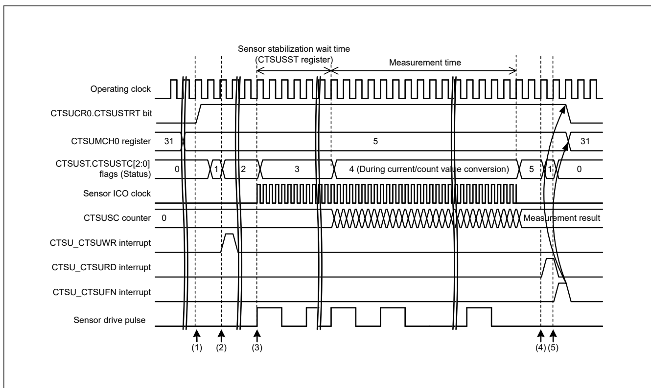
Figure 46.13 Timing of self-capacitance single scan mode when the measurement start condition is a software trigger
