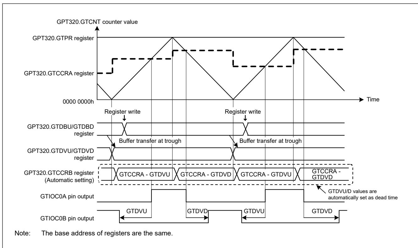
Figure 21.27 Example of automatic compare-match value setting function with dead time in triangle-wave PWM mode 2 or 3, and active-high
