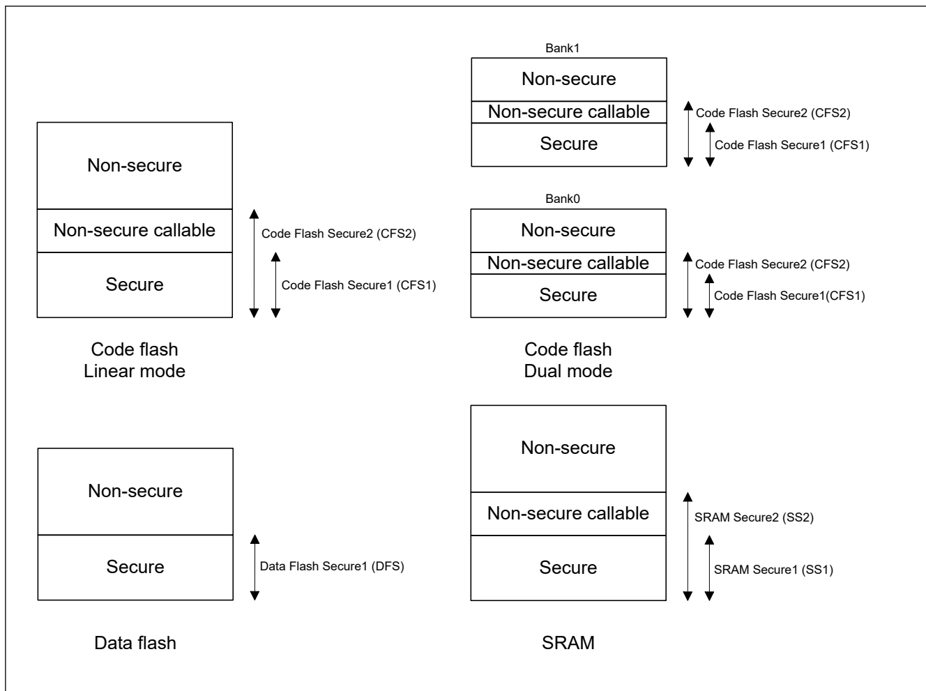
Figure 52.1 Memory mapping
