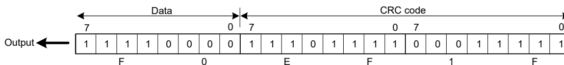
Figure 40.3 MSB-first data transmission
