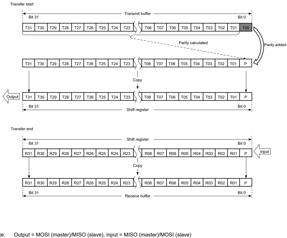
Figure 34.18 MSB-first transfer with 32-bit data and parity enabled
