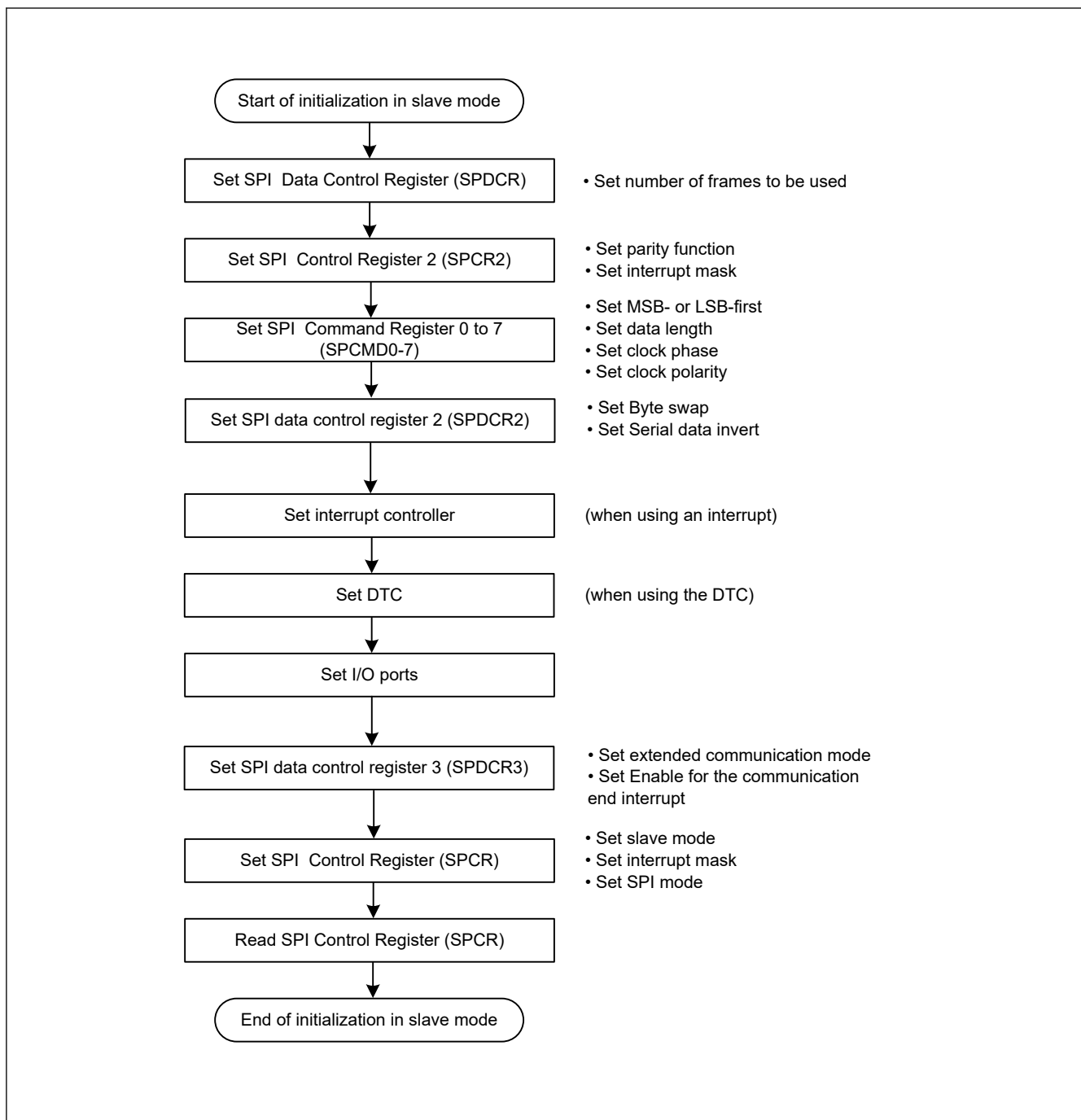
Figure 34.60 Example of initialization flow in slave mode for clock synchronous operation
