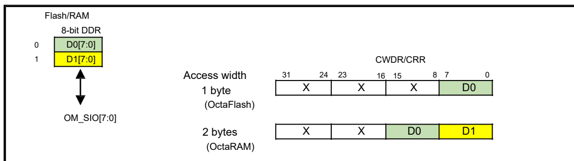
Figure 36.12 Configuration Register Data Alignment in the OctaFlash and OctaRAM Spaces
