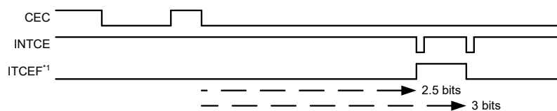
Figure 37.29 Using ITCEF to check INTCE generation source when CECCTL1.CESEL[1:0] = 00b
