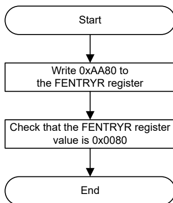
Figure 50.11 Procedure to transition to data flash P/E mode
