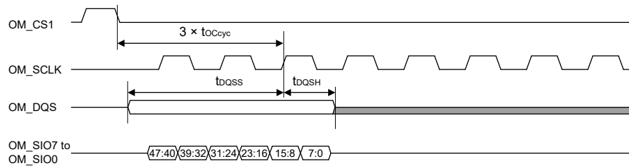
Figure 53.56 DQS Refresh input Timing (OctaRAM™ Read/Write)
