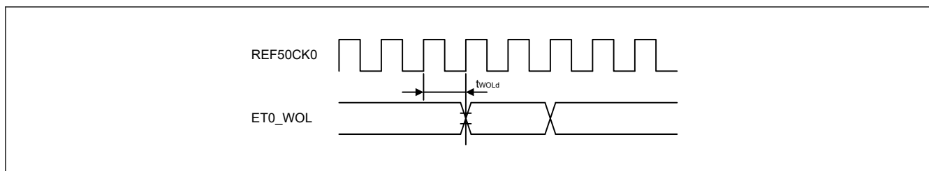
Figure 53.68 WOL output timing for RMII
