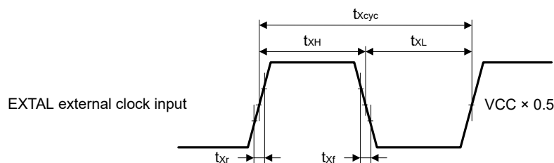
Figure 53.8 EXTAL external clock input timing
