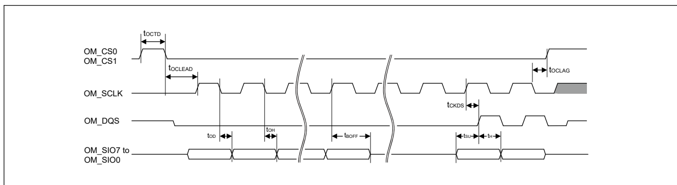
Figure 53.53 SOPI Transfer Format Transmission and Reception Timing
