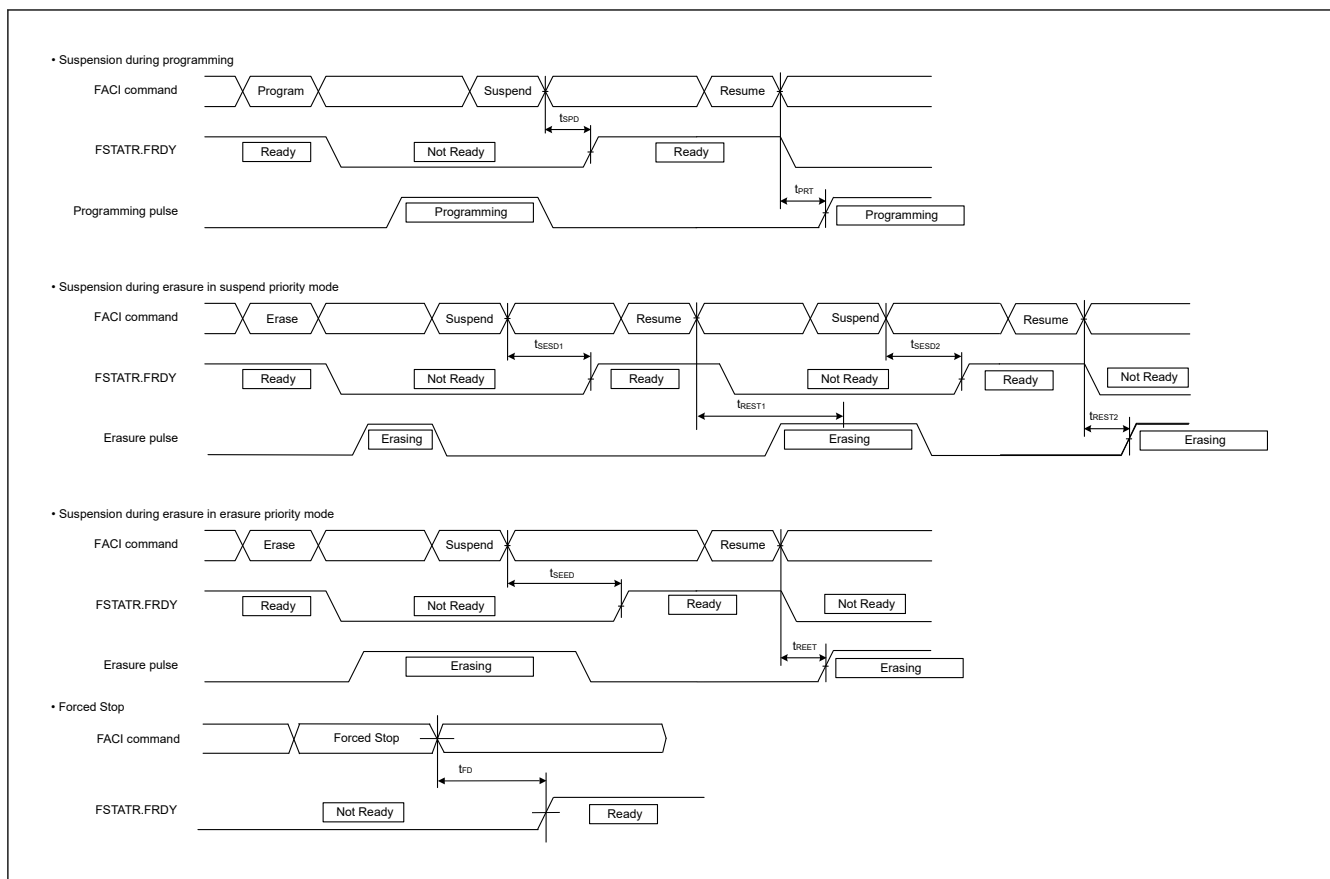
Figure 53.94 Suspension and forced stop timing for flash memory programming and erasure
