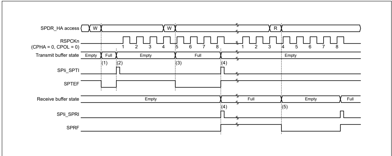
Figure 34.29 Operation example of the SPli_SPTI and SPli_SPRI interrupts when CPHA = 0 and CPOL = 0 in master mode
