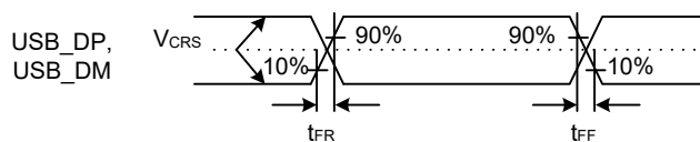
Figure 53.76 USB_DP and USB_DM output timing in full-speed mode
