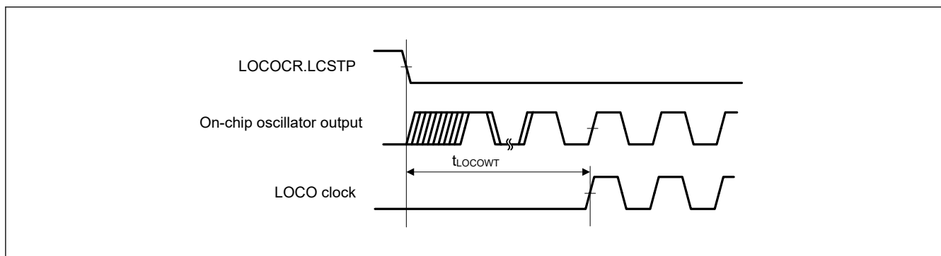
Figure 53.10 LOCO clock oscillation start timing
