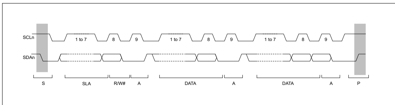
Figure 31.4 I 2 C bus timing when the SLA setting = 7 bits
