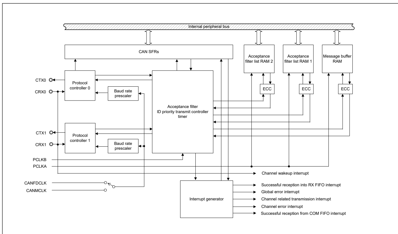
Figure 32.1 Overview of the CAN-FD module
