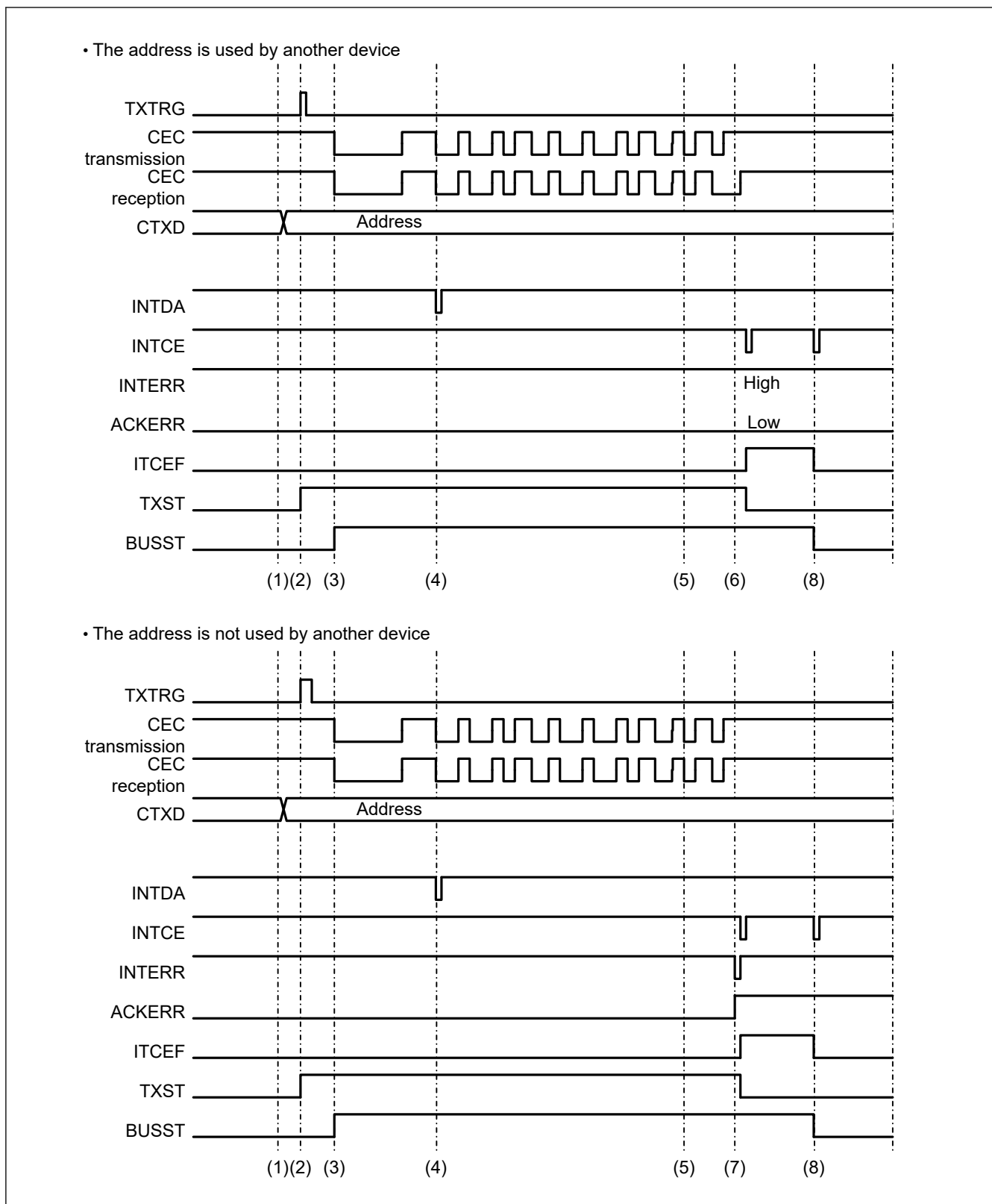
Figure 37.15 Logical allocation (CECCTL1.CESEL[1:0] = 00b)
