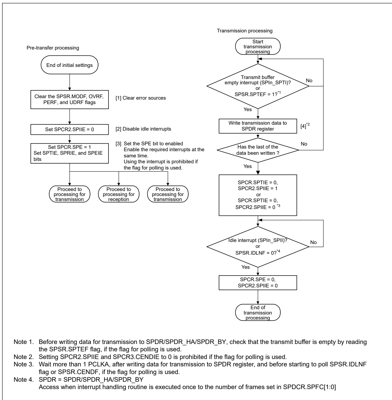
Figure 34.49 Transmission flow in master mode
