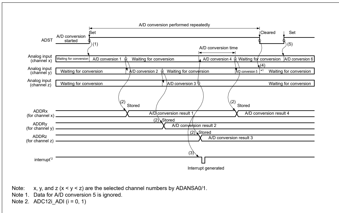
Figure 43.13 Example basic operation in continuous scan mode when the analog inputs (channel x to z) are selected
