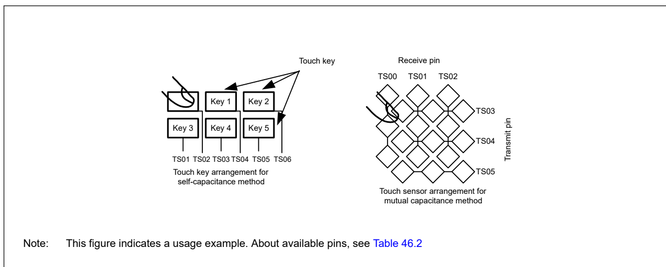
Figure 46.8 Overview of self-capacitance method and mutual capacitance method
