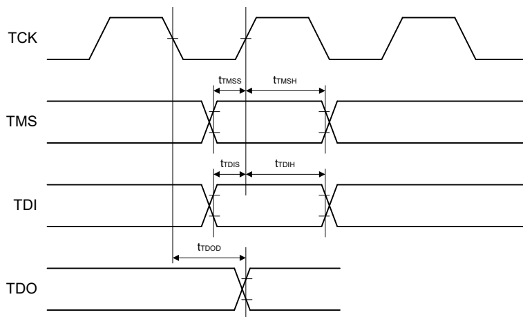
Figure 53.96 Boundary scan input/output timing
