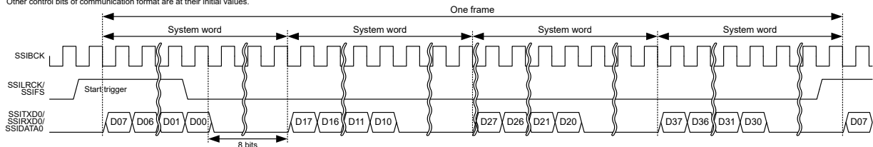
Figure 38.42 TDM format (with padding: system word length > data word length)
