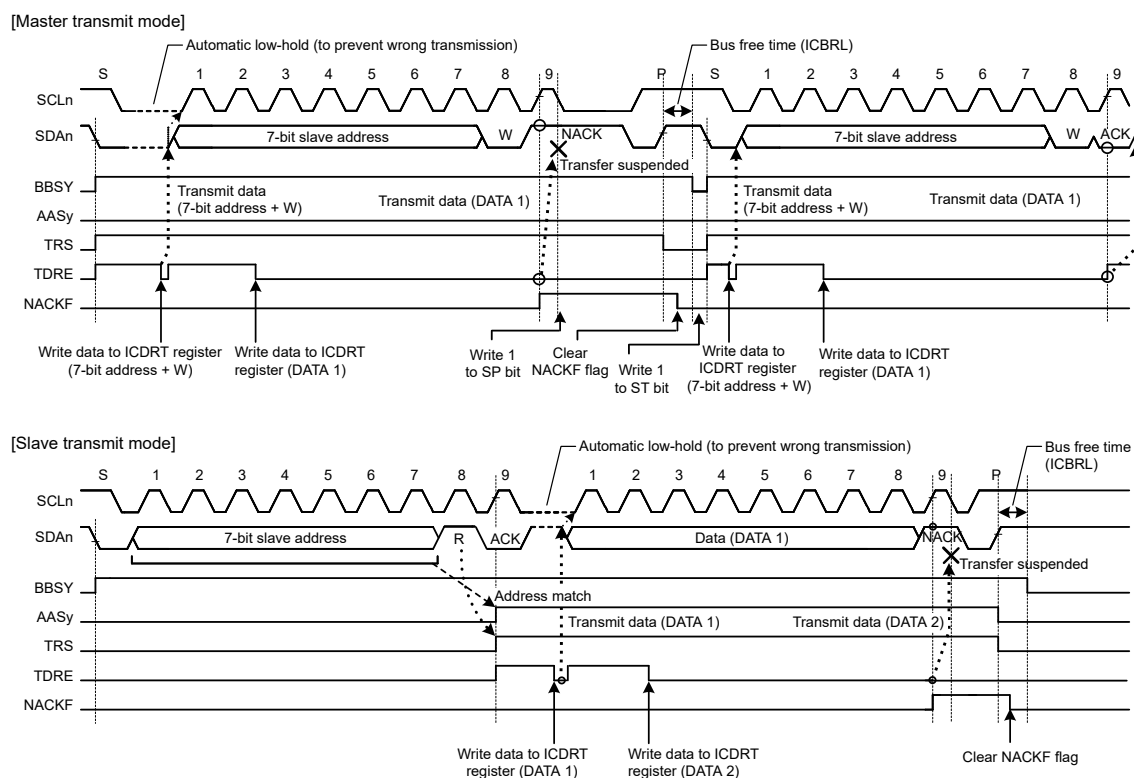
Figure 31.39 Suspension of data transfer when NACK is received, when NACK = 1
