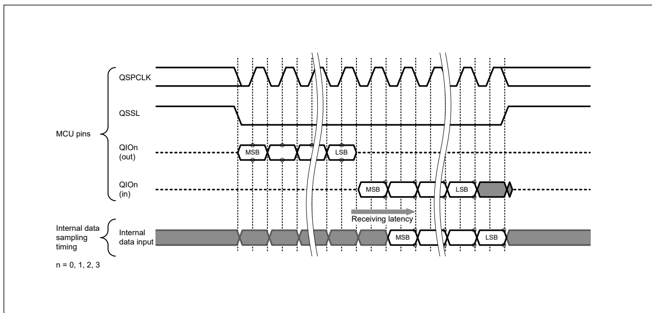
Figure 35.17 Receiving latency
