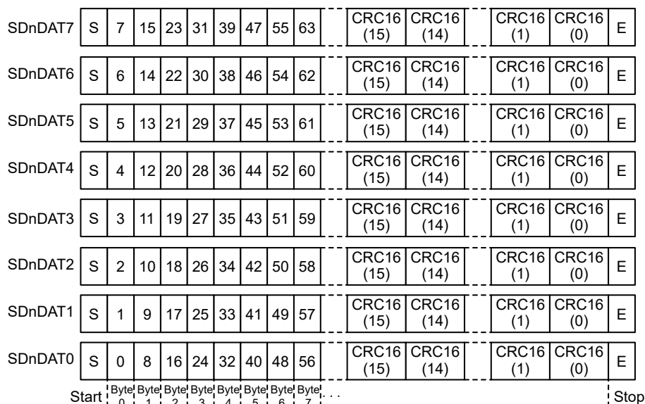
Figure 39.4 SDnDAT in 8-bit width mode
