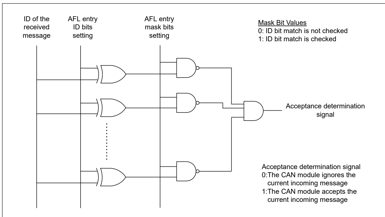
Figure 32.25 Acceptance function
