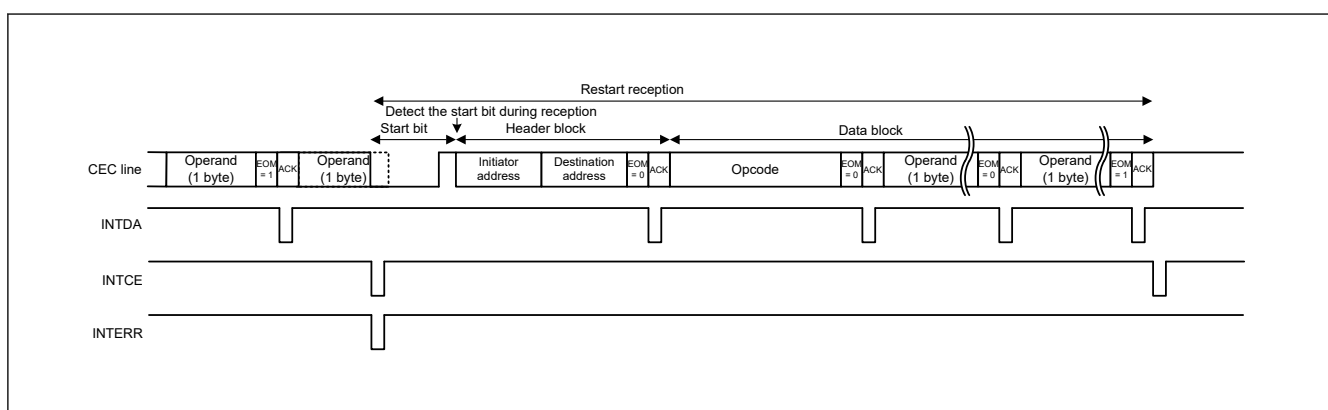
Figure 37.49 Reception restart function operation
