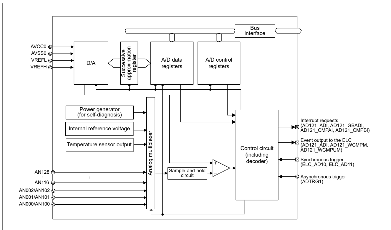
Figure 43.2 ADC12 block diagram (unit 1)
