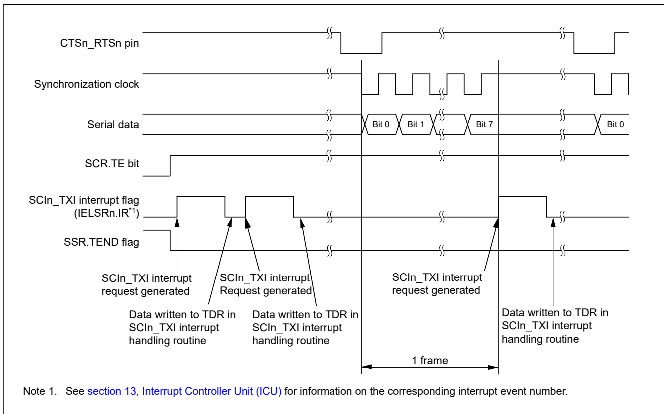
Figure 30.67 Example of serial data transmission in clock synchronous mode when the CTS function is used at the beginning of transmission
