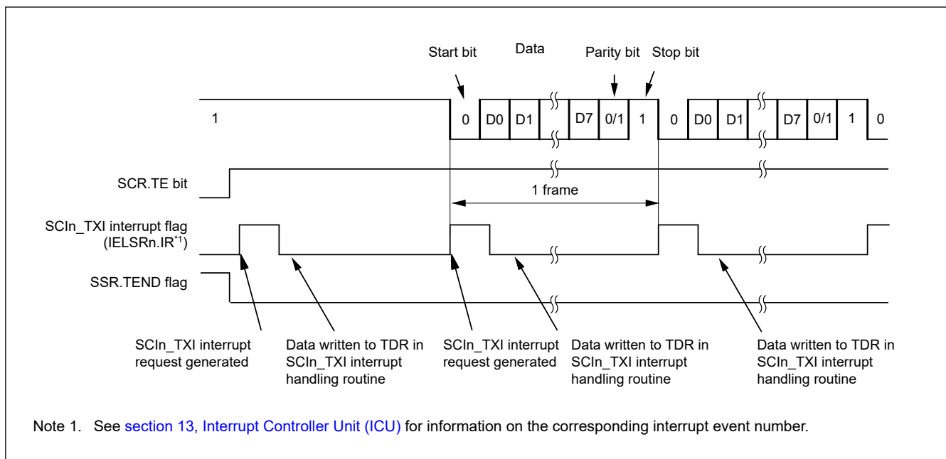
Figure 30.11 Example operation for serial transmission in asynchronous mode (1) with 8-bit data, parity bit, 1 stop bit, CTS function not used, and at the beginning of transmission
