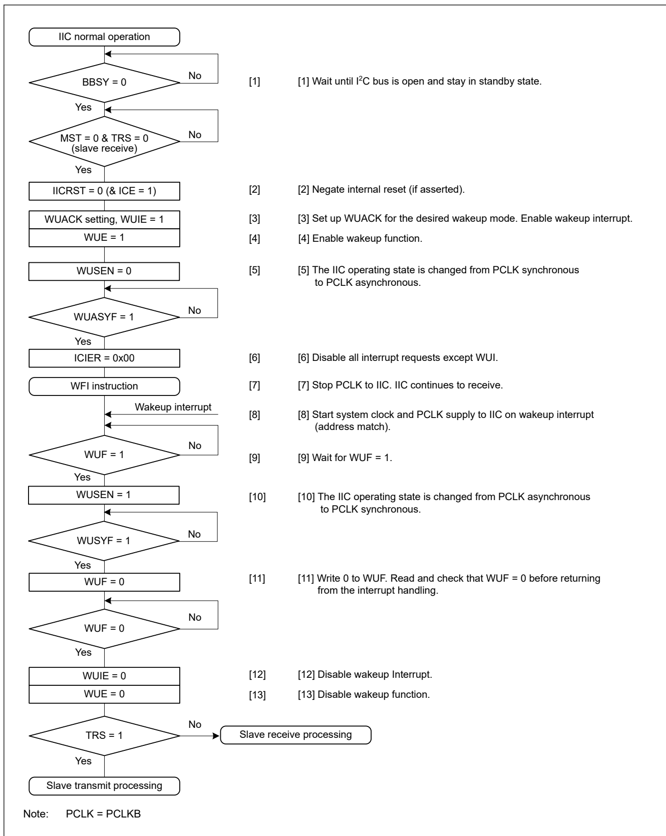
Figure 31.30 Example operation of normal wakeup mode 1 when wakeup is triggered by a wakeup interrupt on match of the slave address
