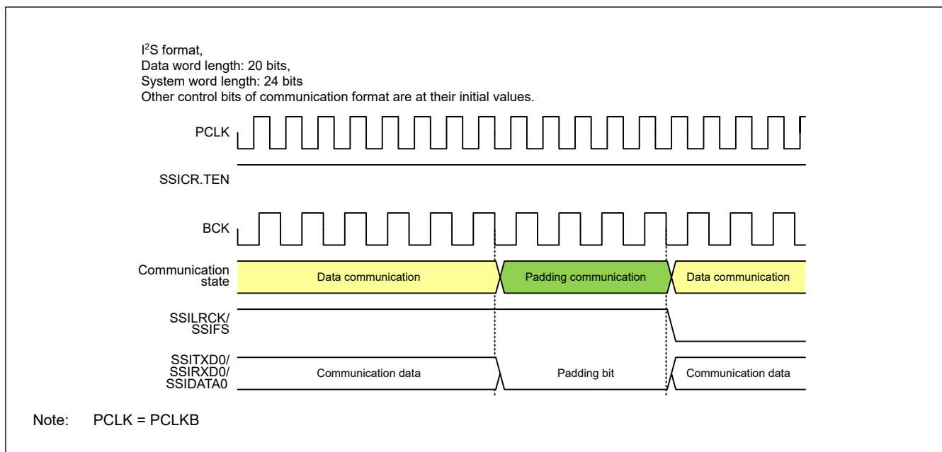
Figure 38.49 Transition from data communication to padding communication
