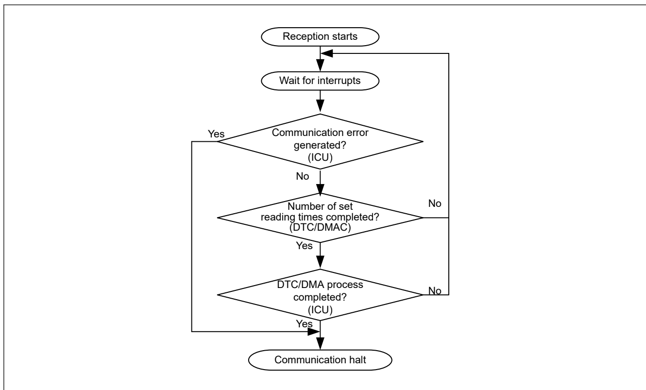
Figure 38.55 Reception procedure
