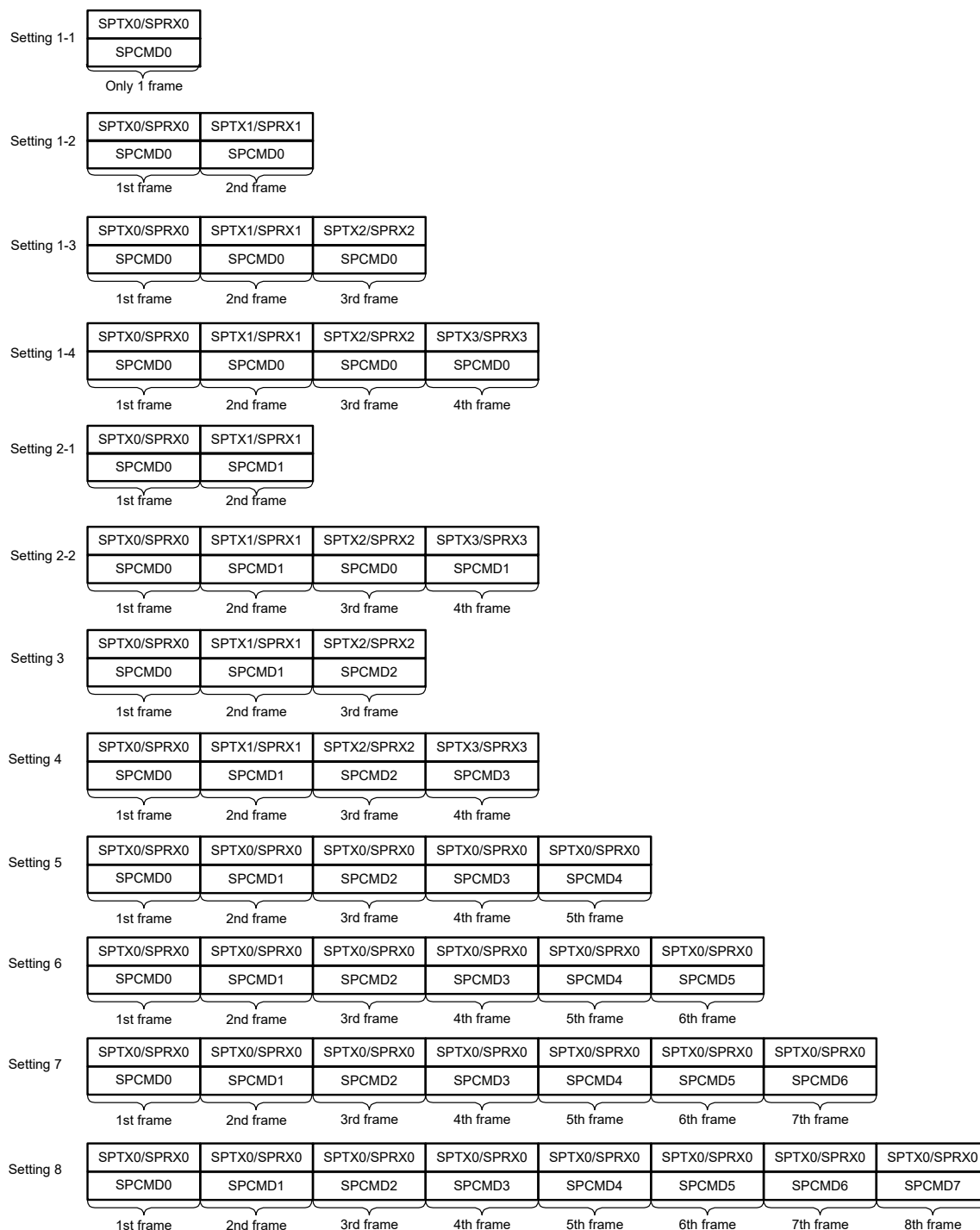
Figure 34.58 Correspondence between SPI Command Register and transmit and receive buffers in sequence operations
