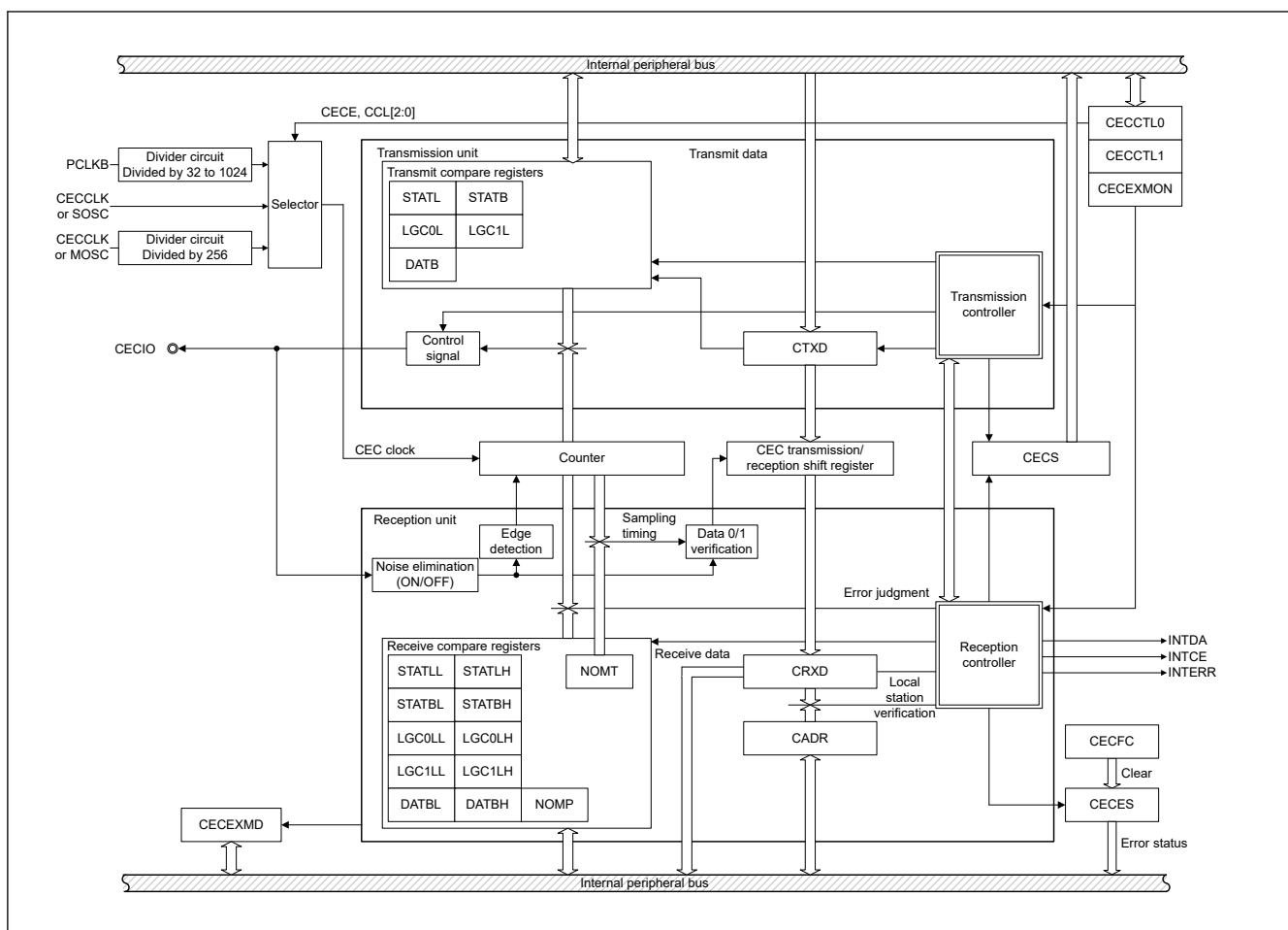
Figure 37.1 CEC block diagram
