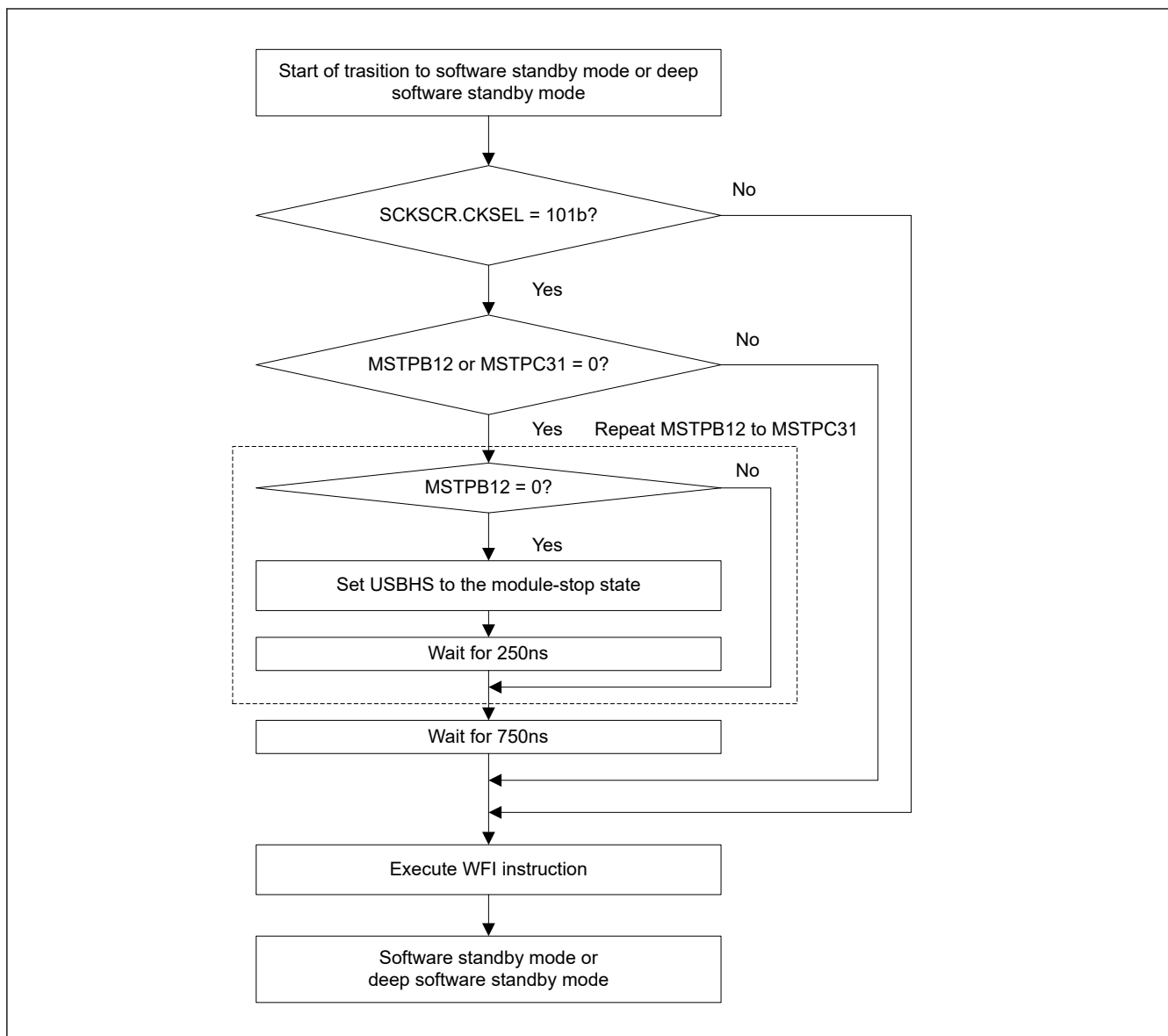
Figure 10.2 Example flow for transition to software standby mode or deep software standby mode
