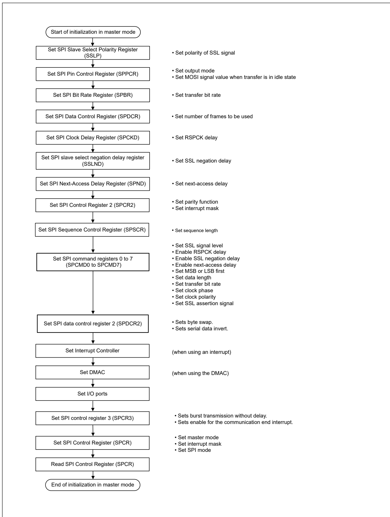
Figure 34.48 Example of initialization flow in master mode for SPI operation
