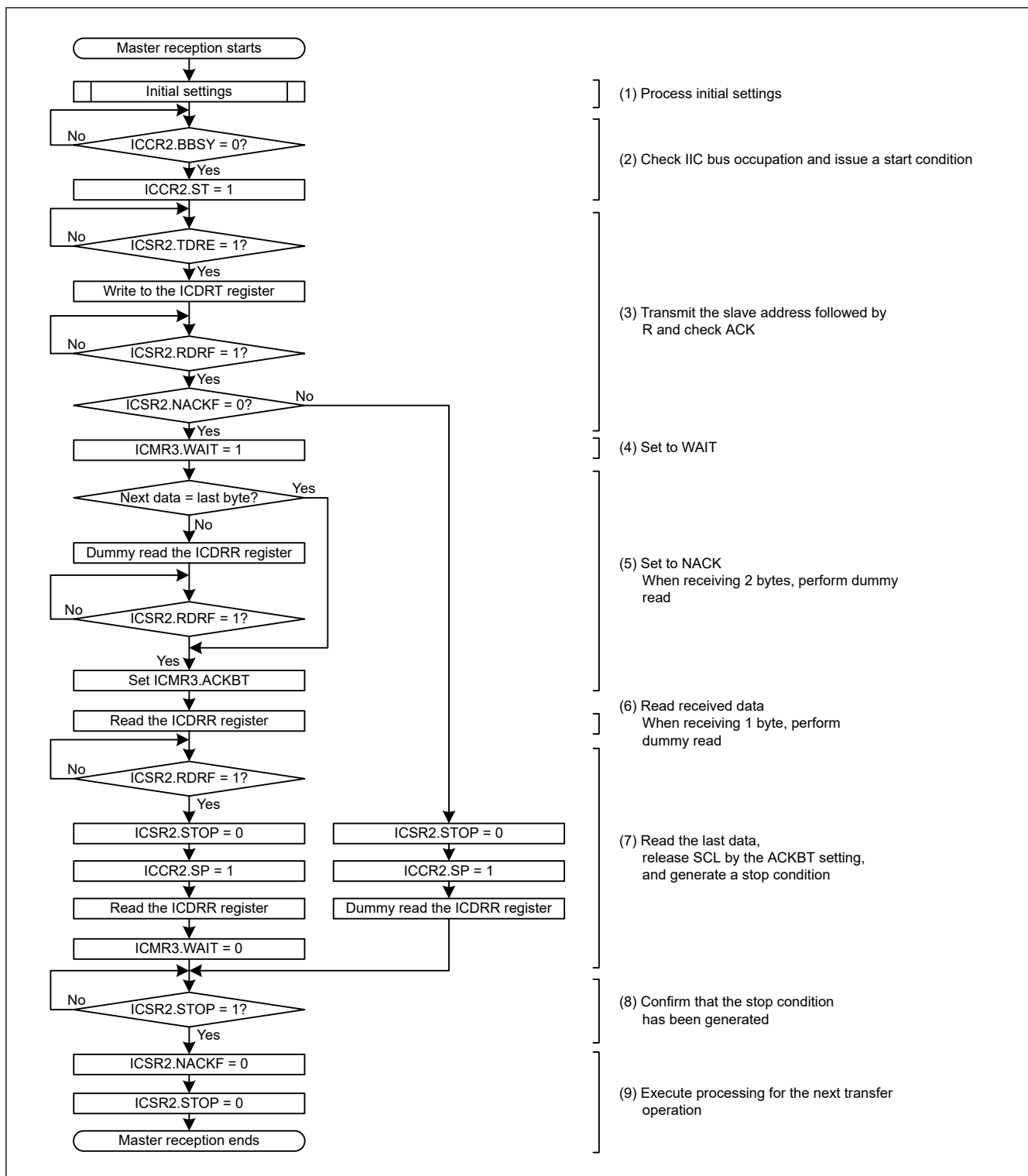
Figure 31.10 Example master reception flow with 7-bit address format of 1 byte or 2 bytes
