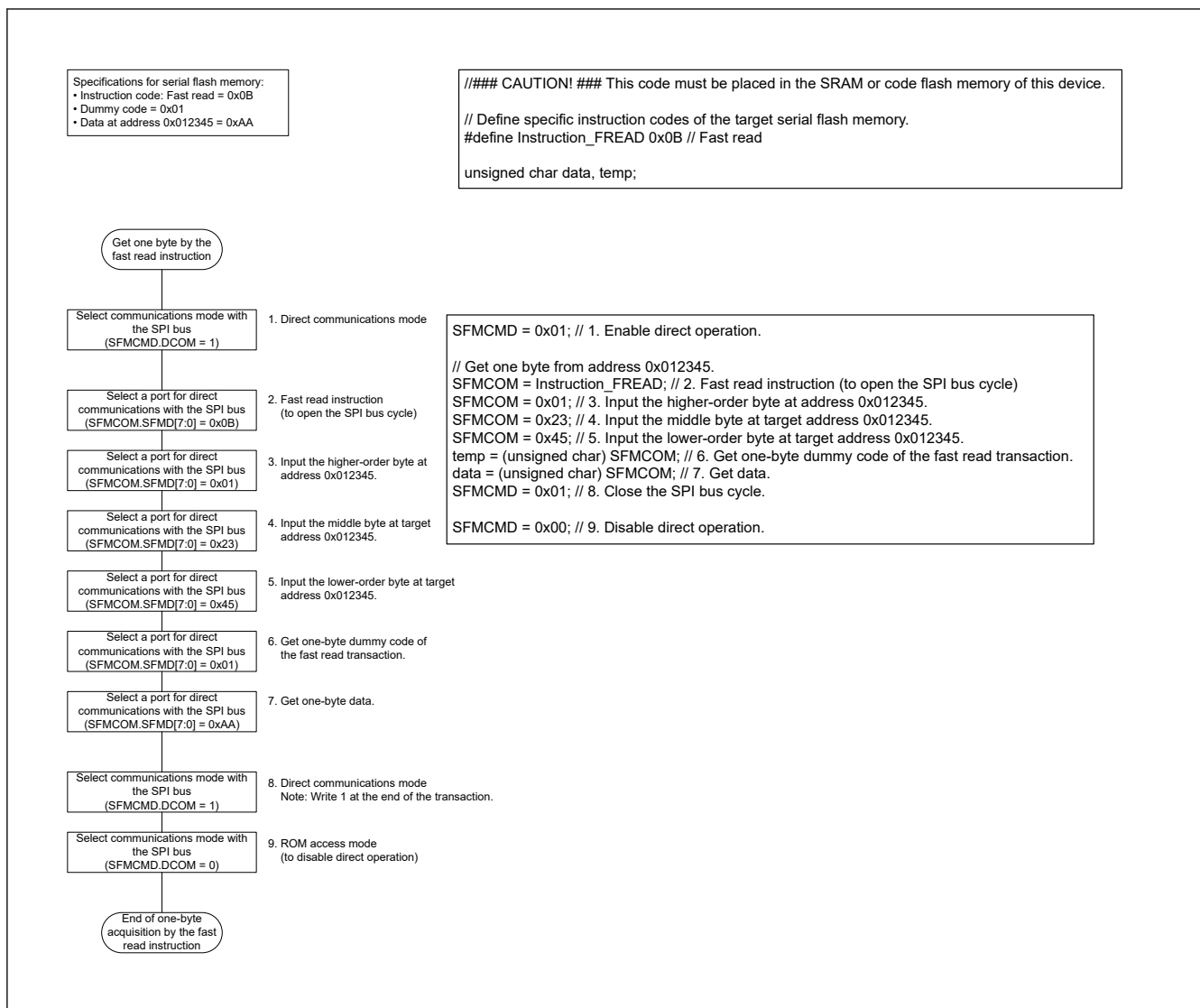
Figure 35.39 Flowchart of One-byte Acquisition by the Fast Read Instruction
