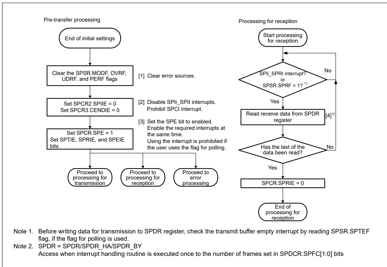
Figure 34.53 Transmission flow in slave mode
