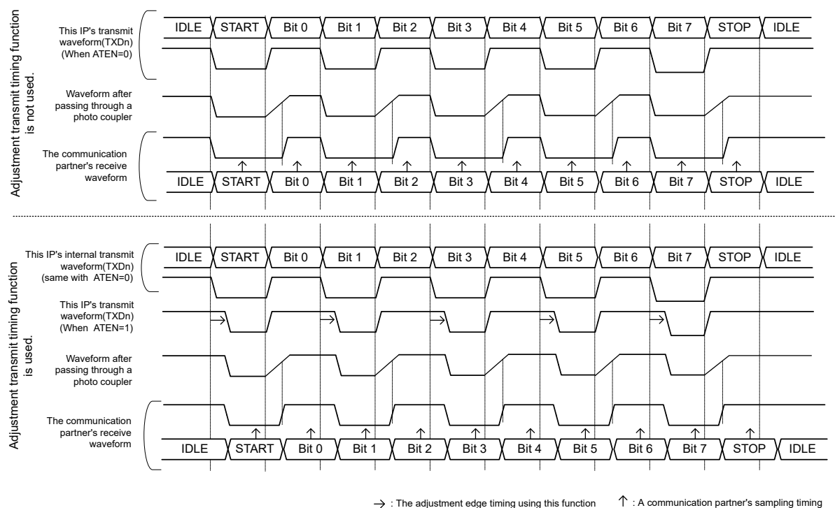
Figure 30.37 The explanation for the transmit waveform through a photo coupler
