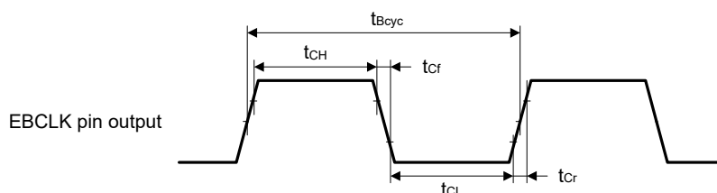
Figure 53.7 EBCLK output timing
