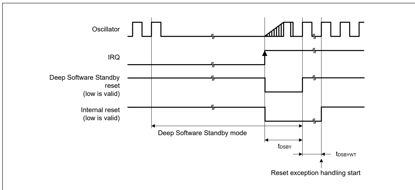
Figure 53.16 Deep Software Standby mode cancellation timing
