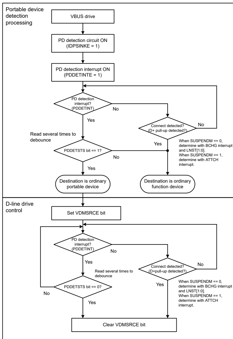
Figure 29.21 Processing flow as charging downstream port with hardware portable device detection function
