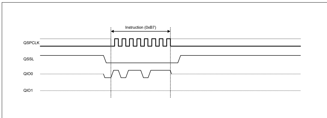
Figure 35.29 Enter 4-Byte Mode bus cycle
