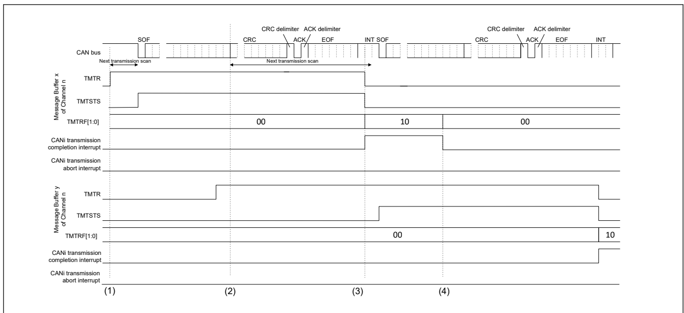
Figure 32.42 Timing of request and flag bits for successful transmission
