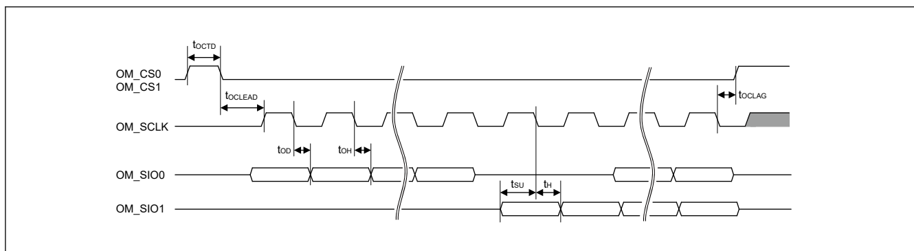
Figure 53.52 SPI Transfer Format Transmission and Reception Timing
