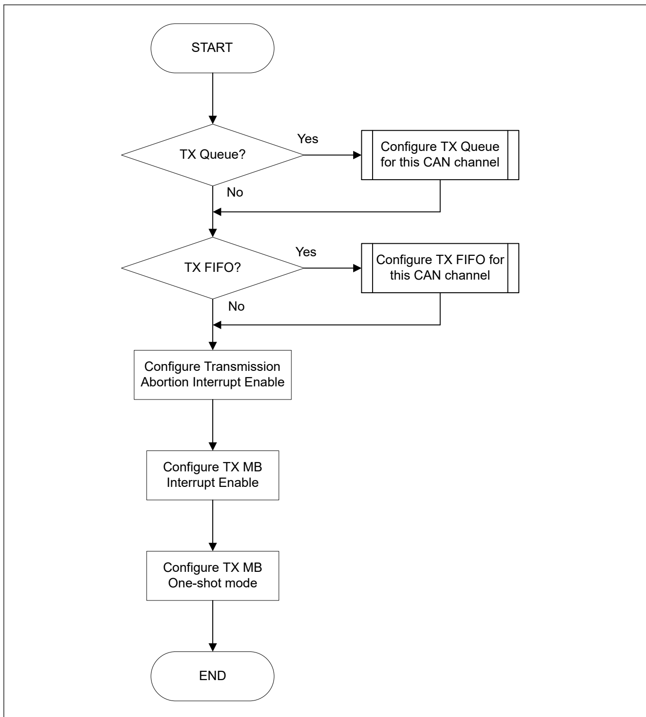
Figure 32.40 Flow for transmission configuration
