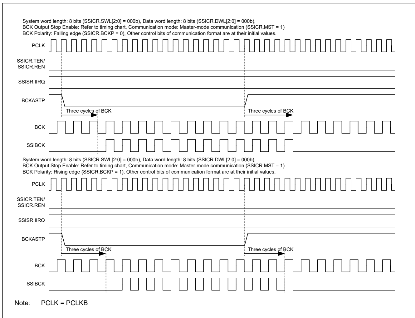
Figure 38.34 Example operation of the BCKASTP bit (idle state)
