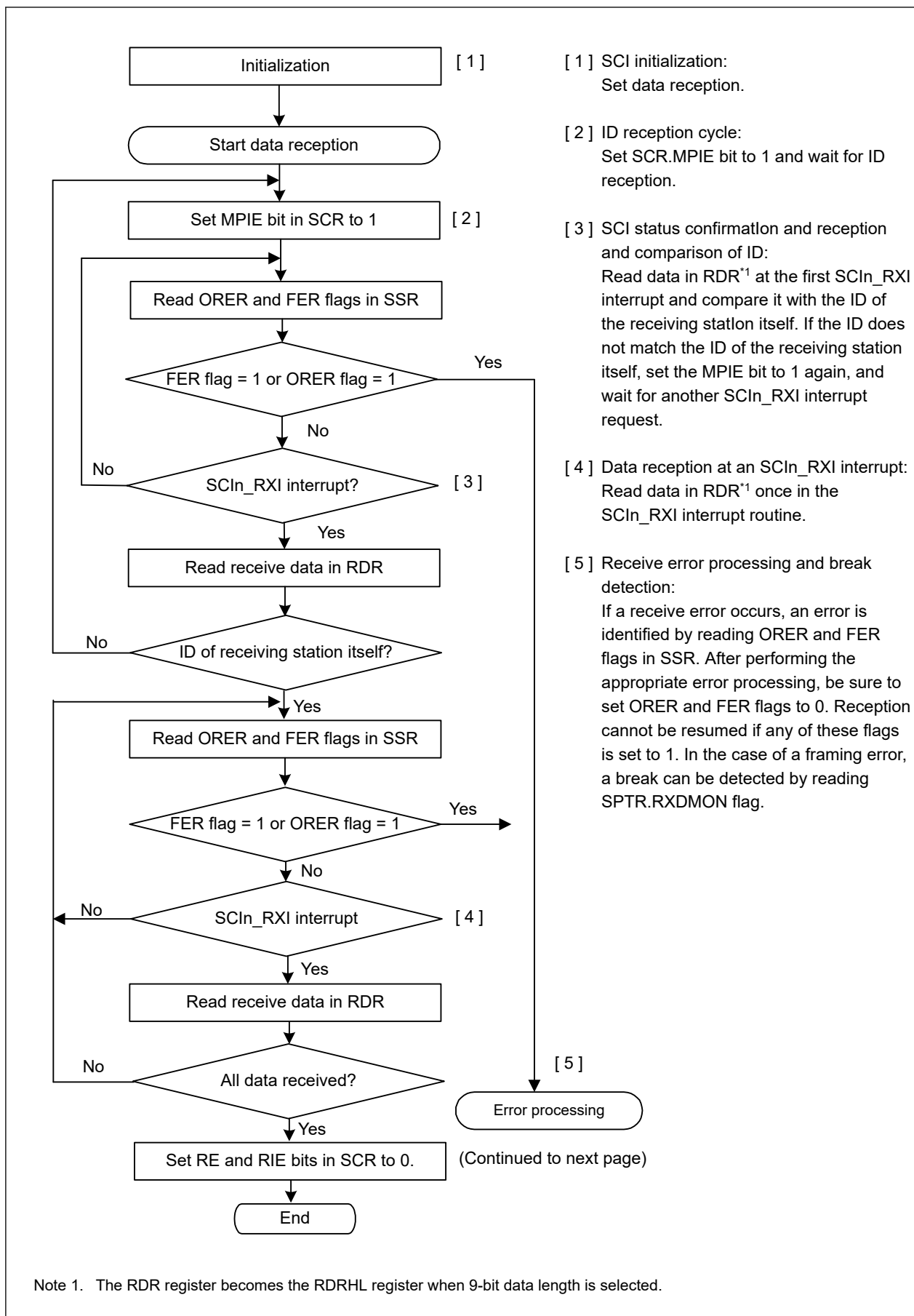
Figure 30.45 Example flow of multi-processor serial reception with non-FIFO selected (1)
