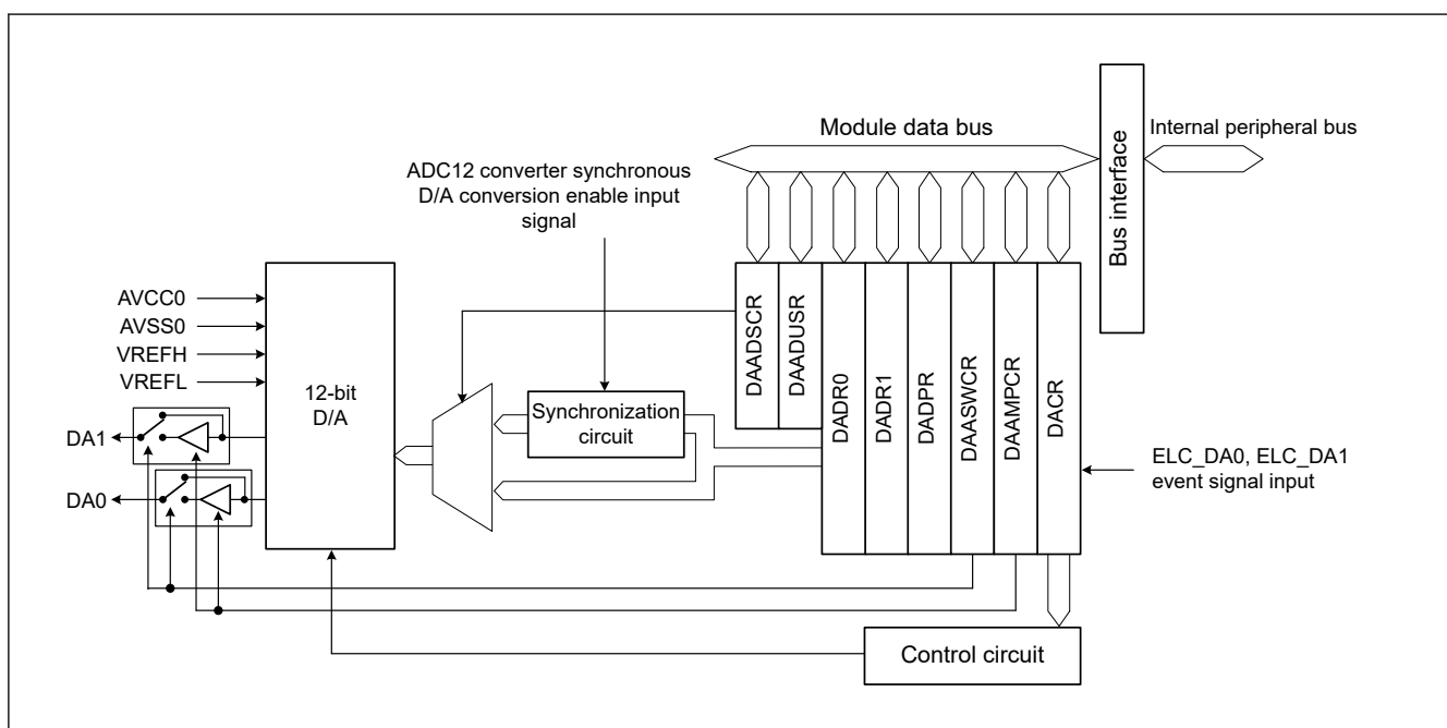
Figure 44.1 DAC12 block diagram
