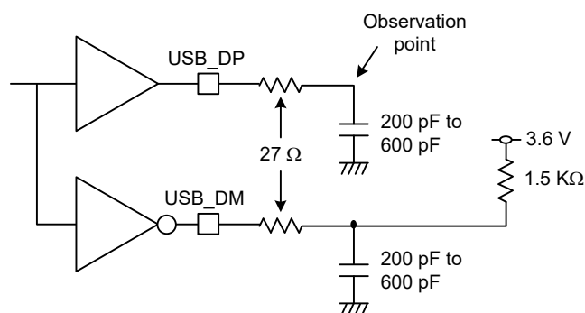
Figure 53.79 Test circuit in low-speed mode
