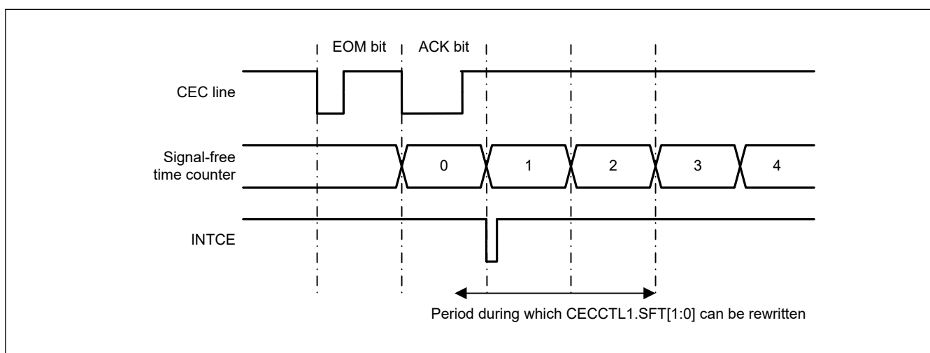
Figure 37.47 Period during which CECCTL1.SFT[1:0] can be rewritten while counting signal-free time
