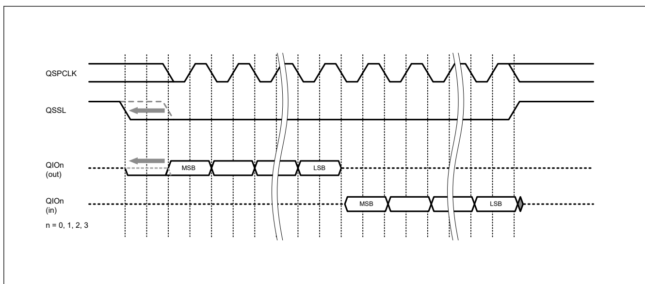
Figure 35.11 Setup time adjustment for the QSSL signal using the SFMSLD bit
