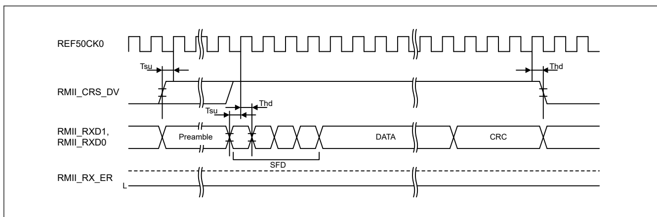
Figure 53.66 RMII reception timing in normal operation
