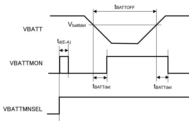
Figure 53.93 Battery backup function characteristics
