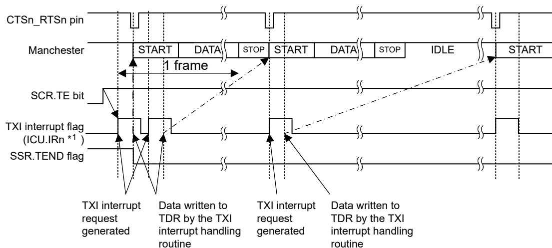
Figure 30.57 Example of Start-of-Transmission Operation for Serial Transmission in Manchester Mode (Without Preface but with the CTS Function)
