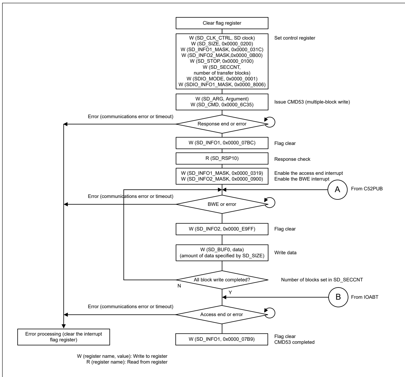
Figure 39.20 Example of IO_RW_EXTENDED command during a CMD53 multiple block write operation
