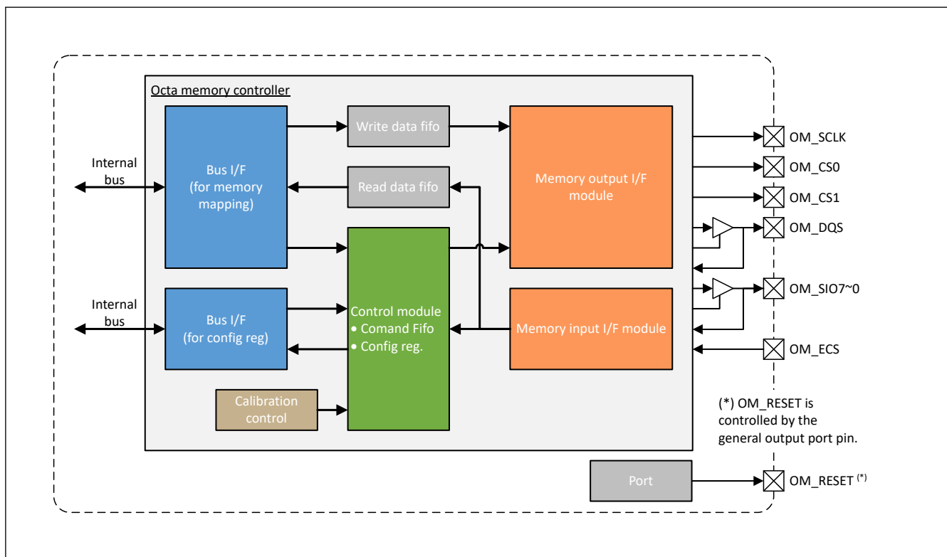
Figure 36.1 Block diagram
