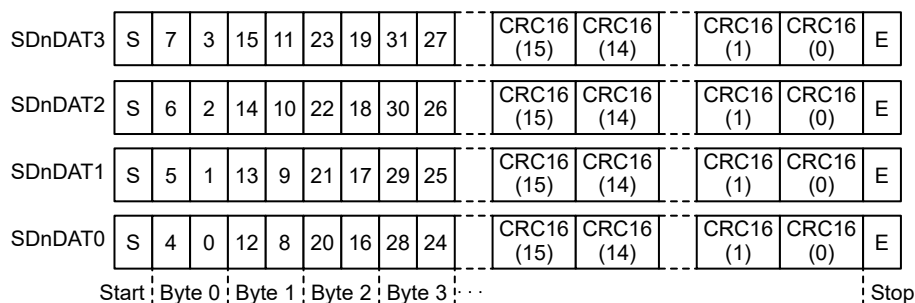
Figure 39.3 SDnDAT in 4-bit width mode
