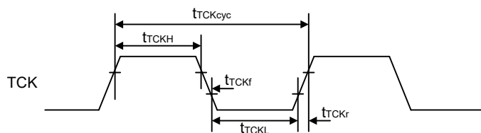
Figure 53.95 Boundary scan TCK timing
