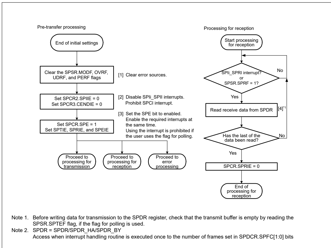
Figure 34.54 Reception flow in slave mode
