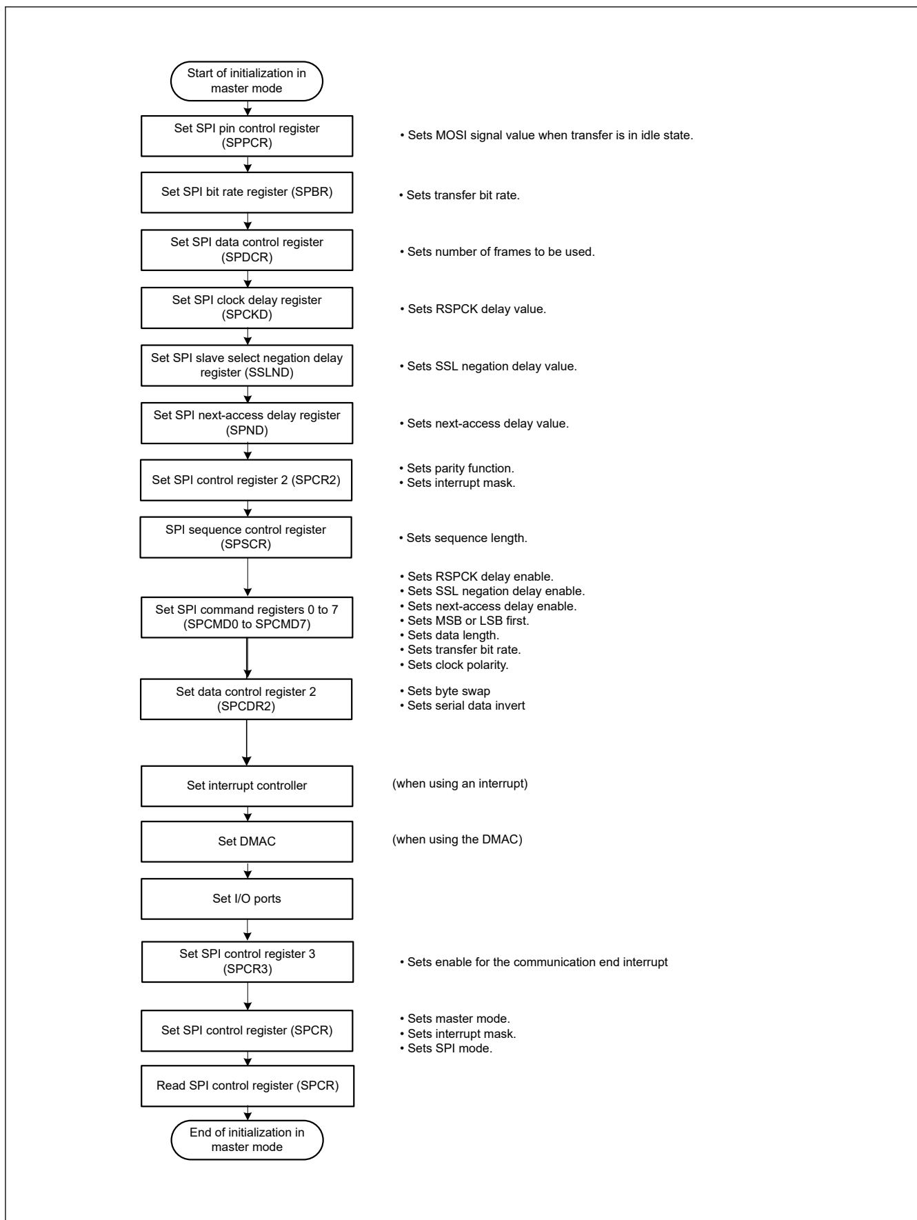
Figure 34.59 Example of initialization flow in master mode for clock synchronous operation
