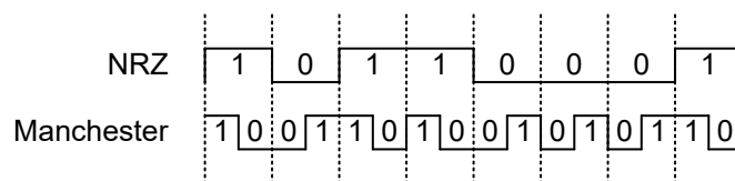
Figure 30.49 Example of Manchester Encoding
