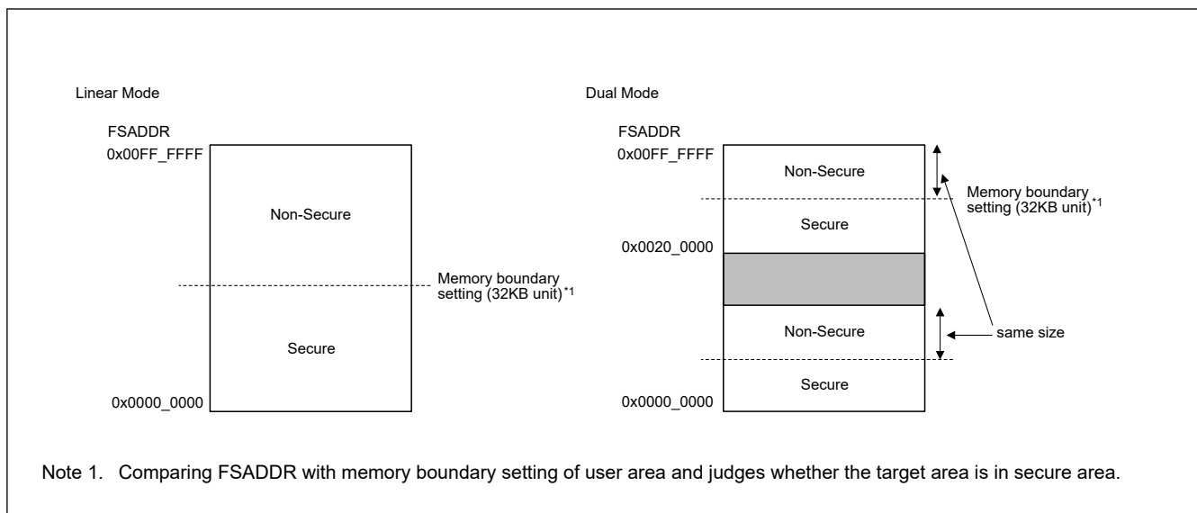
Figure 50.36 Secure/non-secure region in user area
