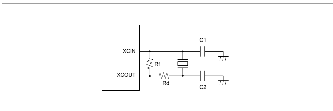
Figure 8.7 Connection example of 32.768-kHz crystal resonator
