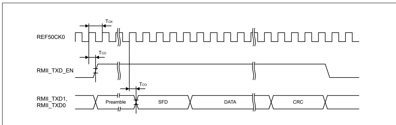
Figure 53.65 RMII transmission timing
