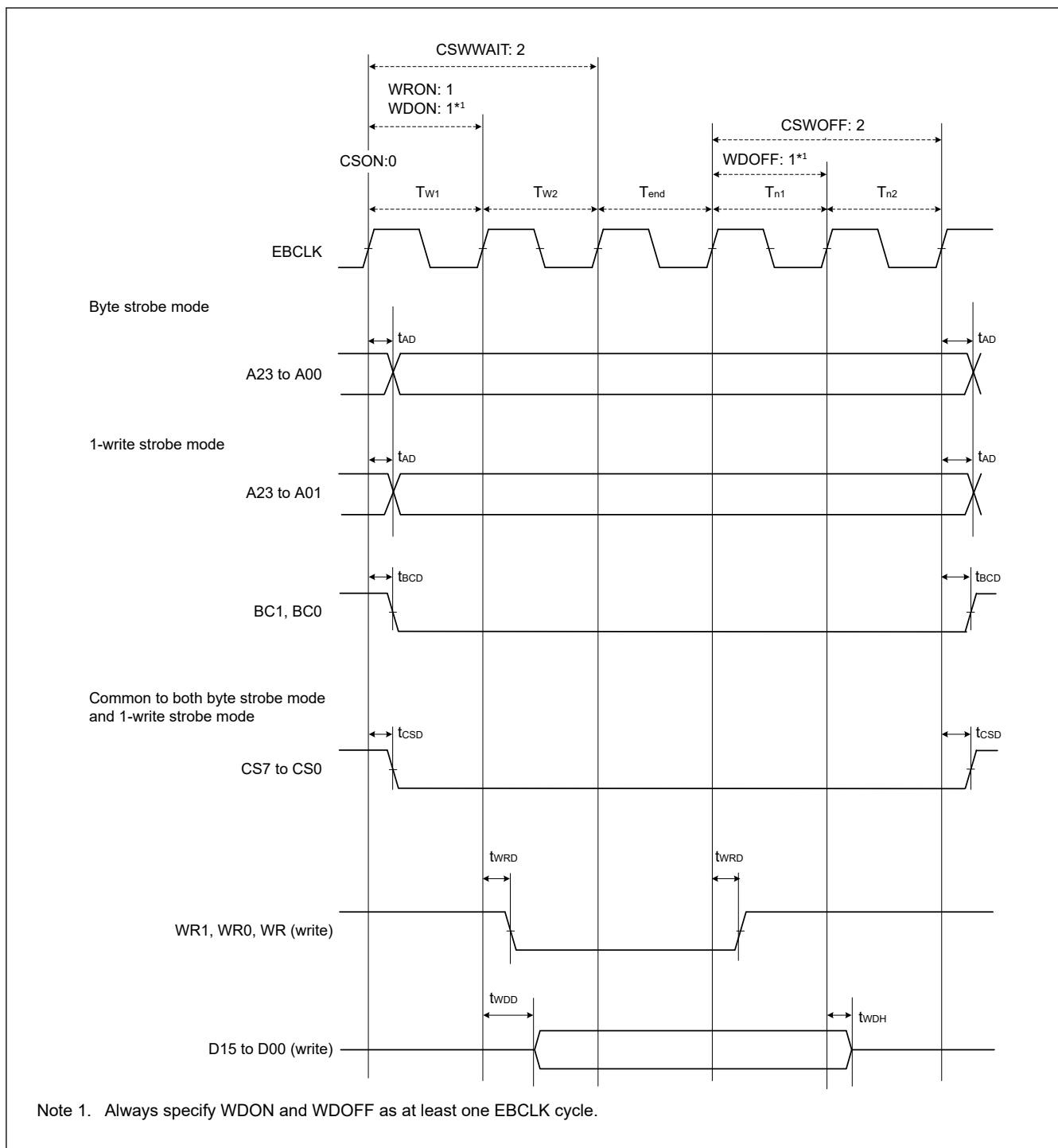
Figure 53.23 External bus timing for normal write cycle with bus clock synchronized
