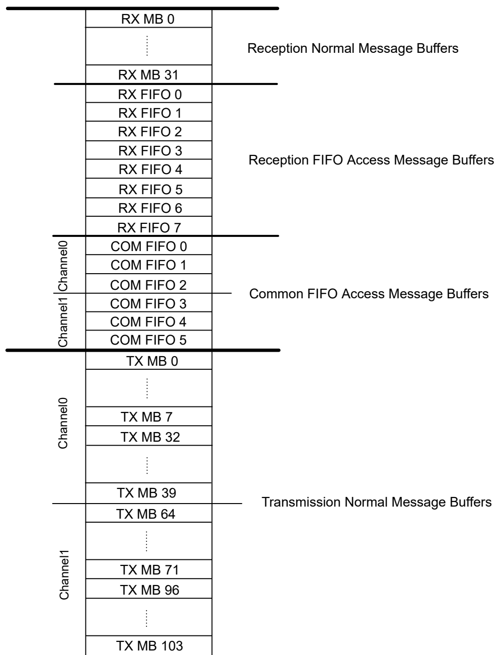
Figure 32.28 Message buffer configuration
