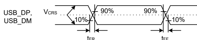
Figure 53.80 USB_DP and USB_DM output timing in full-speed mode
