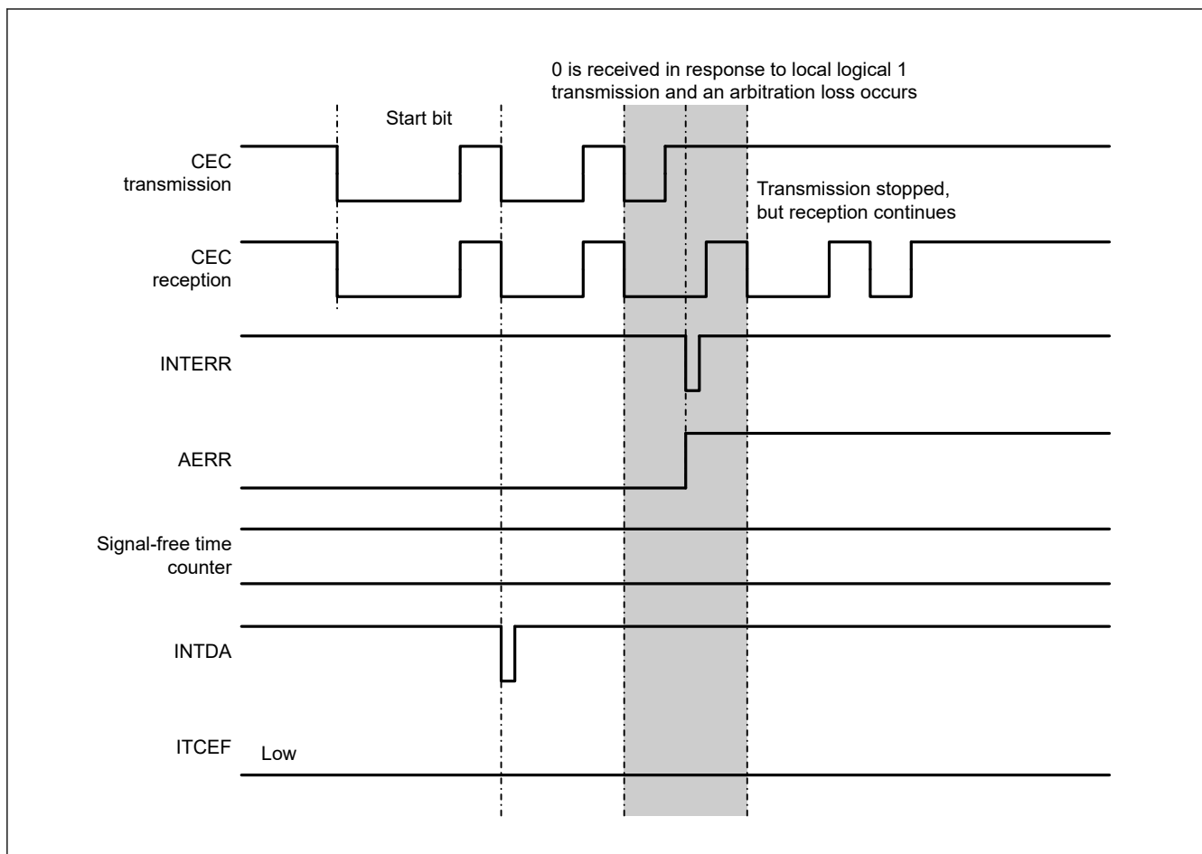
Figure 37.38 Arbitration timing
