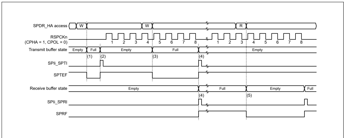
Figure 34.30 Operation example of the SPli_SPTI and SPli_SPRI interrupts when CPHA = 1 and CPOL = 0 in master mode
