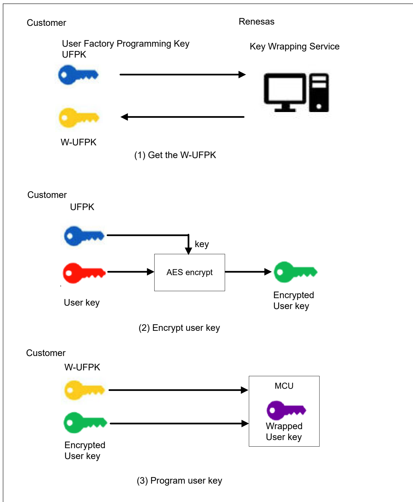
Figure 52.3 Key Injection
