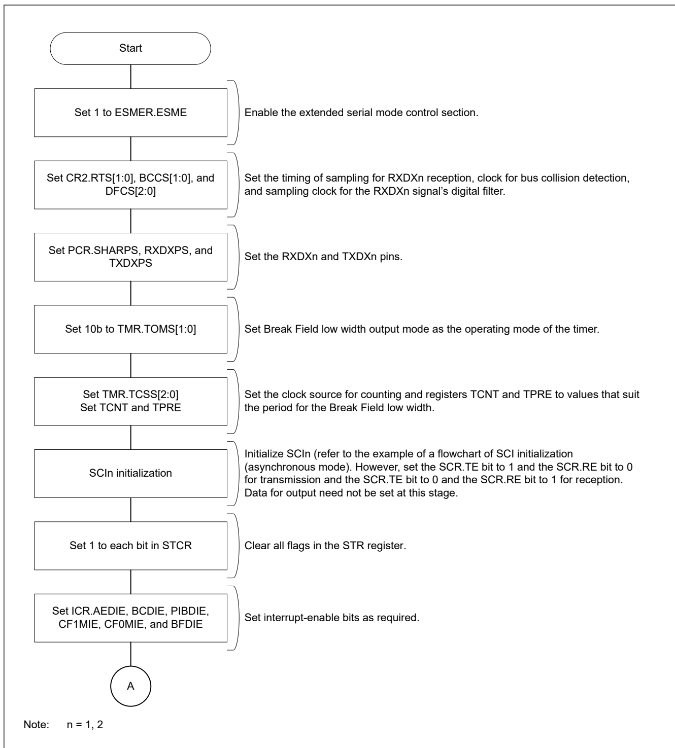
Figure 30.103 Example of Start Frame Transmission (1/2)
