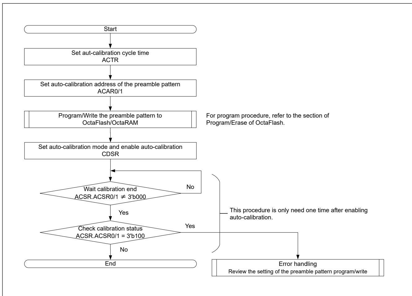
Figure 36.14 Automatic Calibration Setting Flow
