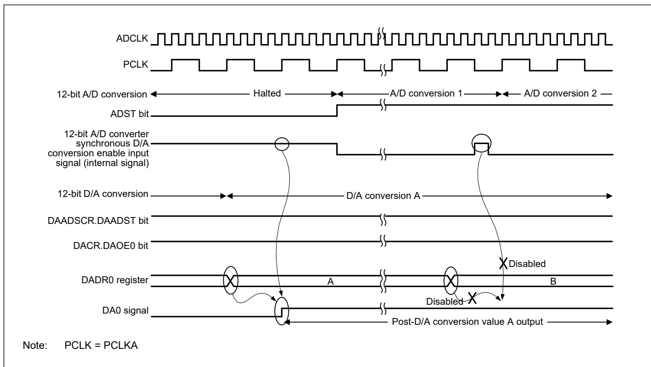
Figure 44.4 Example when the DAC12 cannot capture the synchronous D/A conversion enable input signal from the ADC12 (unit 1)
