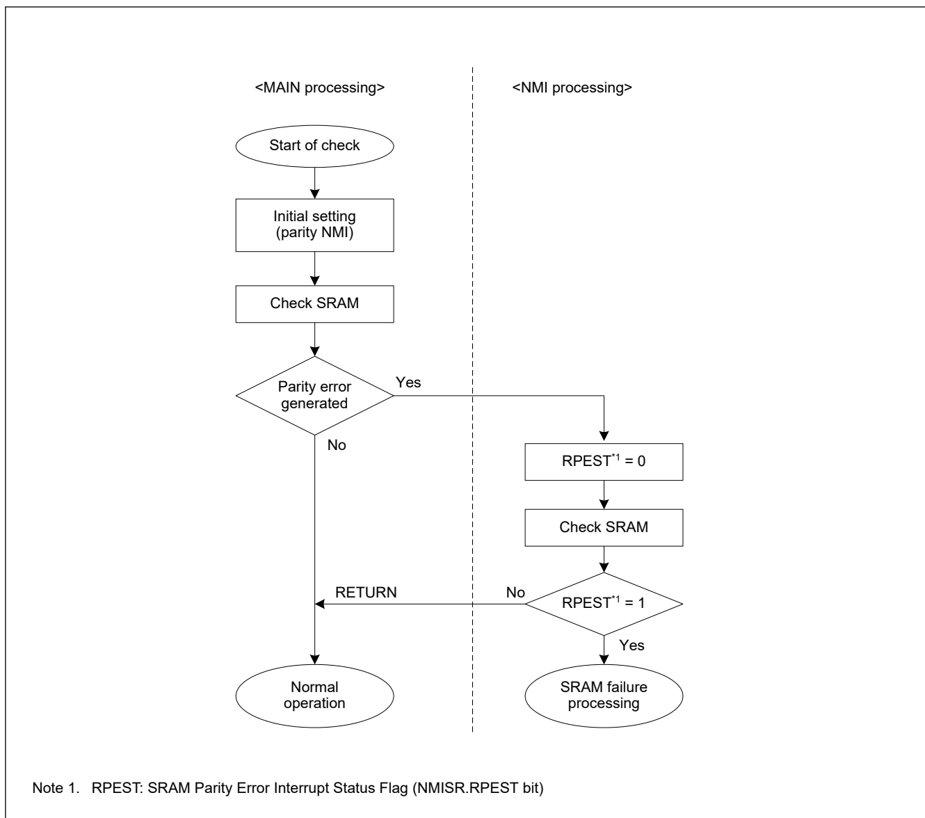
Figure 48.3 Flow of SRAM parity check when SRAM parity interrupt is enabled
