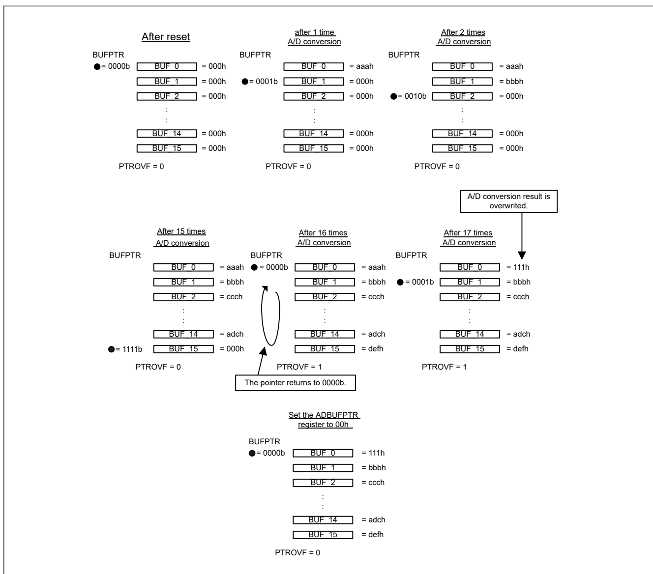
Figure 43.37 Data Buffers, Pointer, and Overflow Flag Operations
