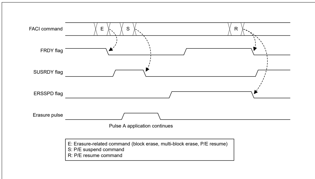
Figure 50.20 Suspension during erasure (eraser priority mode)
