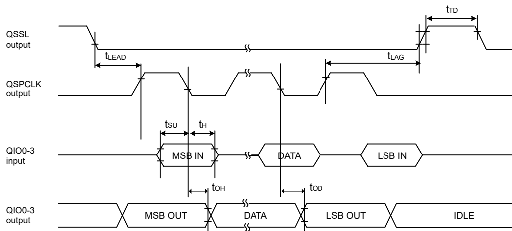
Figure 53.50 Transmit and receive timing
