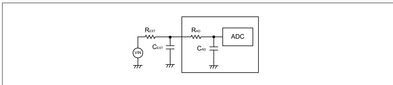
Figure 43.40 Sample and hold circuit simplified diagram
