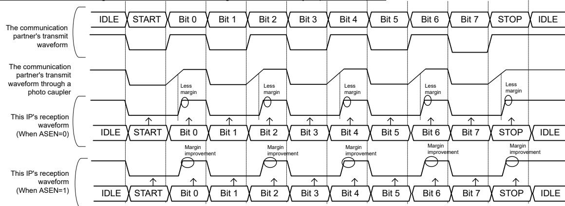
Figure 30.33 Improvement of reception margin when receive sampling timing adjustment function Image
