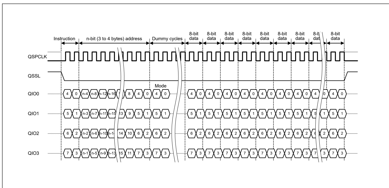
Figure 35.7 Quad SPI protocol example for Fast Read Quad I/O
