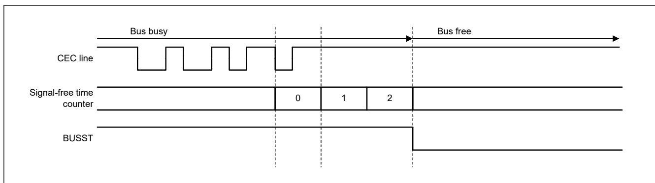
Figure 37.25 Timing when signal-free time set by CECCTL1.SFT[1:0] bits has elapsed after completion of communication
