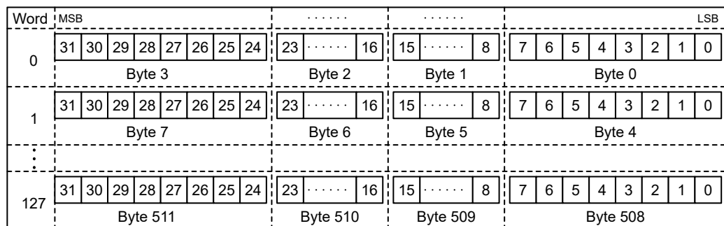
Figure 39.5 SD_BUF store data
