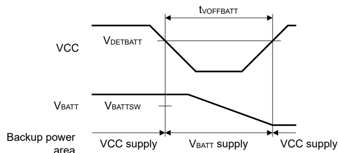
Figure 53.92 Battery backup function characteristics
