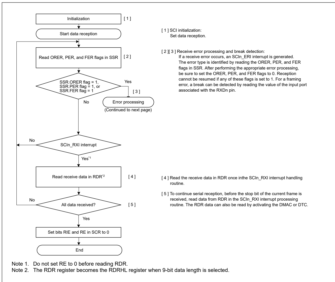
Figure 30.20 Example flow of serial reception in asynchronous mode with non-FIFO selected and Address Matching Disabled (1)
