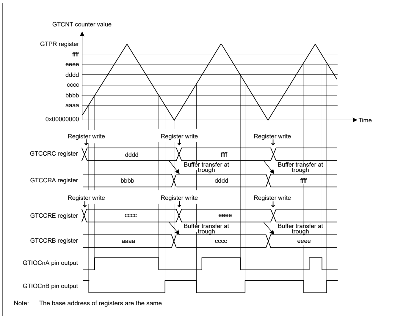
Figure 21.21 Example of triangle-wave PWM mode 1 operation with buffer operation, low output from the GTIOCnA pin and high output from the GTIOCnB pin at count start, output toggled at GTCCRA/GTCCRB register compare match, and output retained at cycle end
