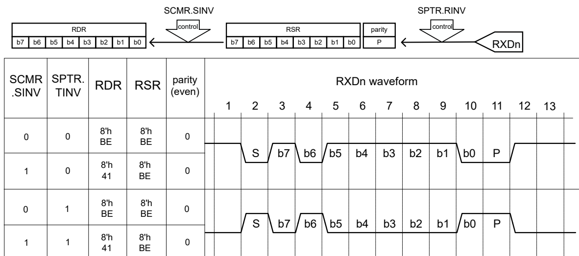
Figure 30.5 Example of the receive/transmit data control
