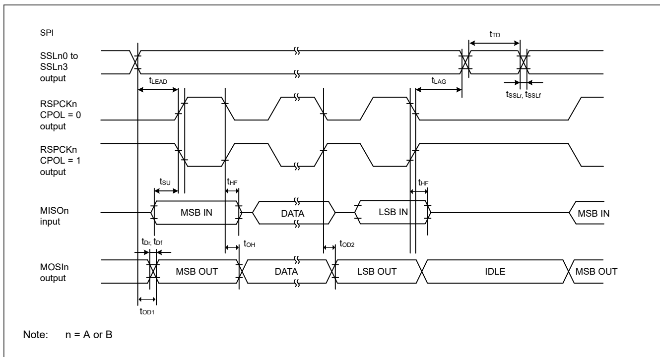
Figure 53.44 SPI timing for master when CPHA = 0 and the bit rate is set to PCLKA/2
