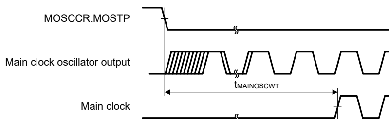
Figure 53.9 Main clock oscillation start timing
