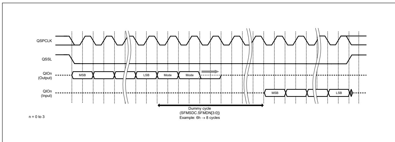
Figure 35.14 Hold Time Adjustment of Output Enabling Using the SFMOEX Bit (Fast Read)
