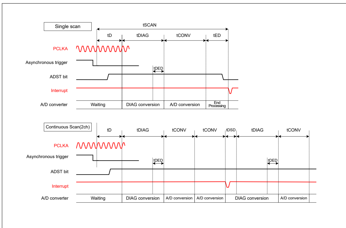
Figure 43.32 Scan conversion timing when activated by an asynchronous trigger input (ADTRG0)
