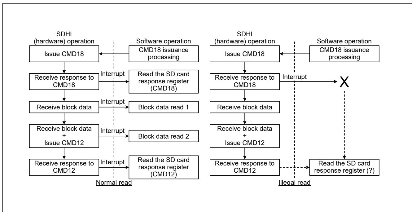
Figure 39.25 Multiple block read operation flow chart (two blocks)
