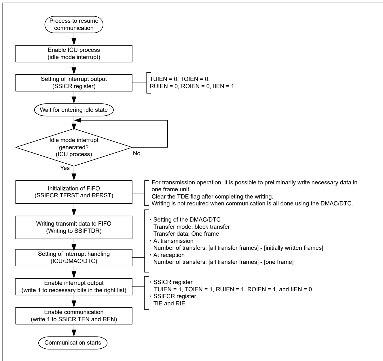
Figure 38.58 Procedure to resume communication (CPU operation procedure)
