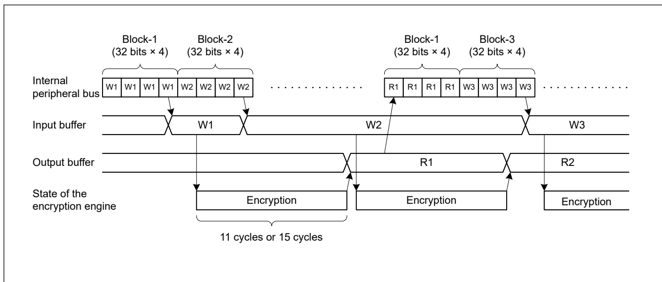
Figure 42.3 Encryption and decryption timing (AES)
