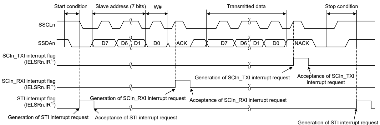
Figure 30.94 Example 2 of operations for master transmission in simple IIC mode with 7-bit slave addresses, ACK interrupts, and NACK interrupts
