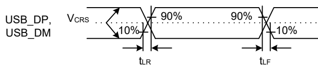
Figure 53.74 USB_DP and USB_DM output timing in low-speed mode
