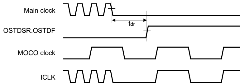
Figure 53.87 Oscillation stop detection timing
