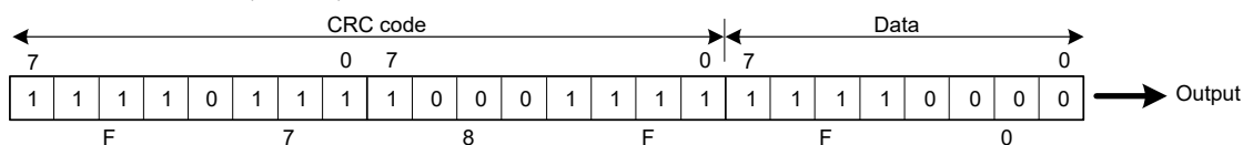
Figure 40.2 LSB-first data transmission
