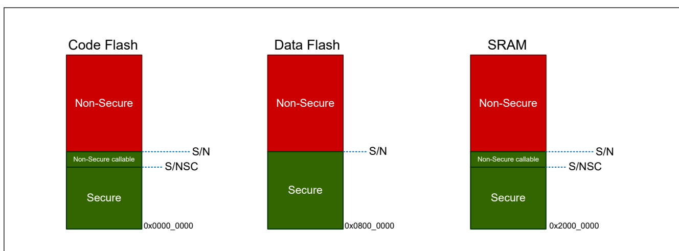
Figure 2.2 Memory partitioning
