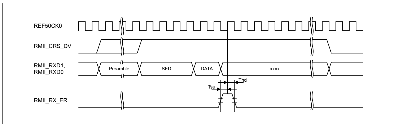
Figure 53.67 RMII reception timing when an error occurs
