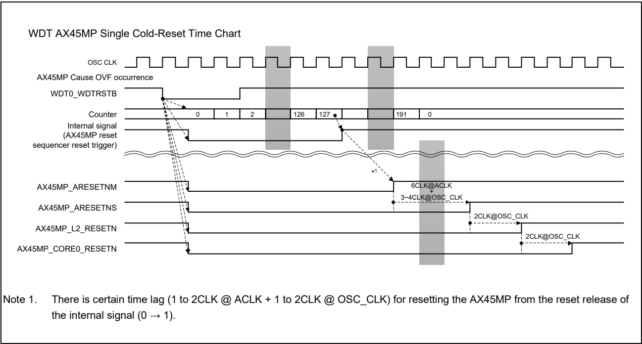
Figure 7.4 Timing of Cold Reset for the AX45MP Alone due to the WDT Source
