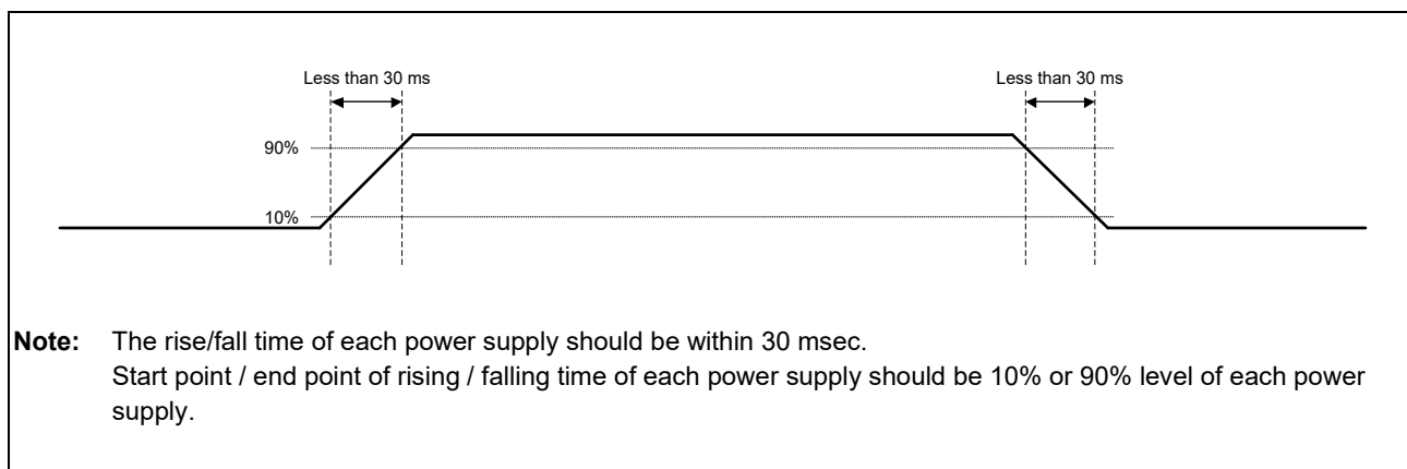
Figure 48.2 Power Up Time/Power Down Time (1)
