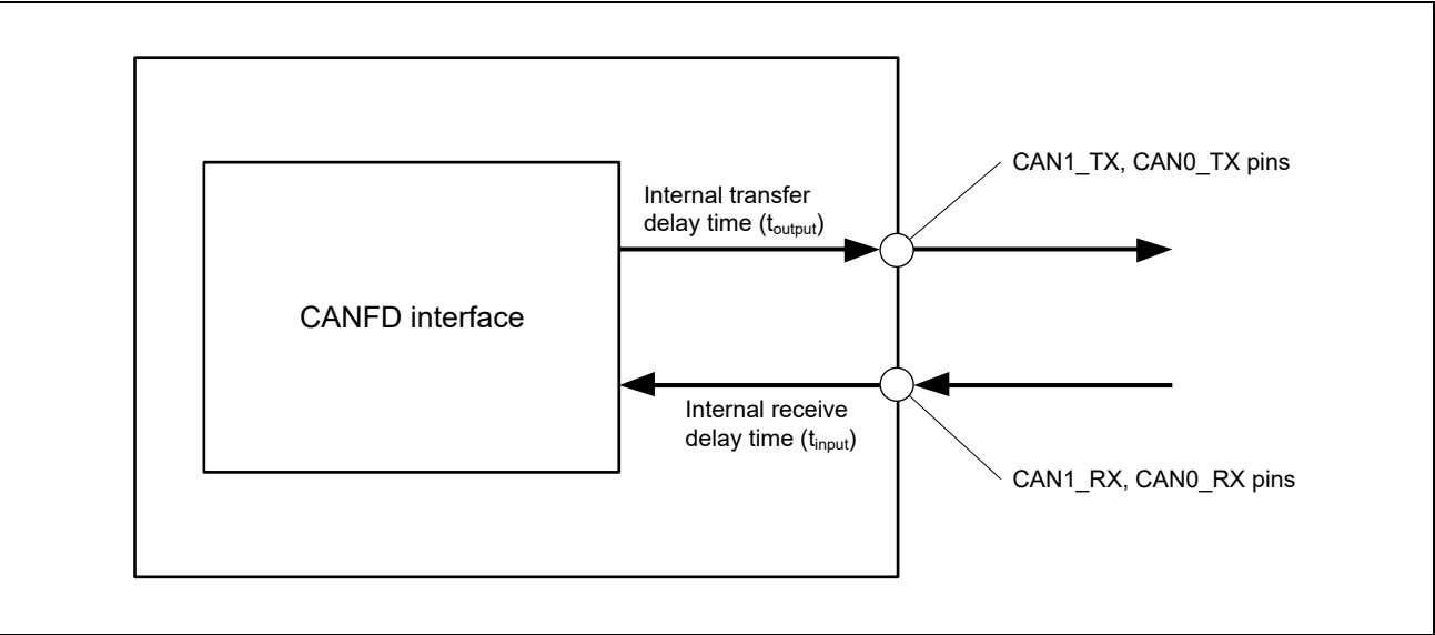
Figure 48.34 CAN-FD Interface Condition
