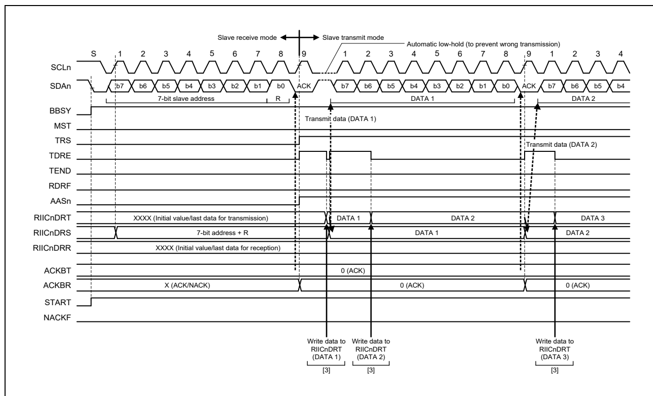
Figure 26.16 Slave Transmit Operation Timing (1) (7-Bit Address Format)
