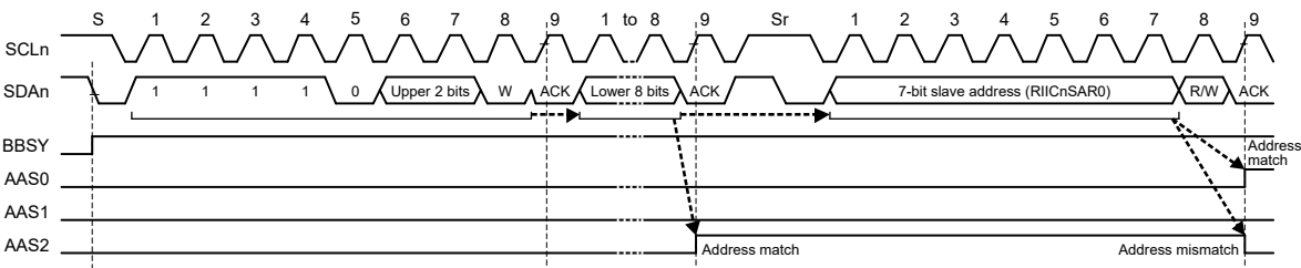
Figure 26.26 AASy Flag Set/Clear Timing with 7-Bit/10-Bit Address Formats Mixed
