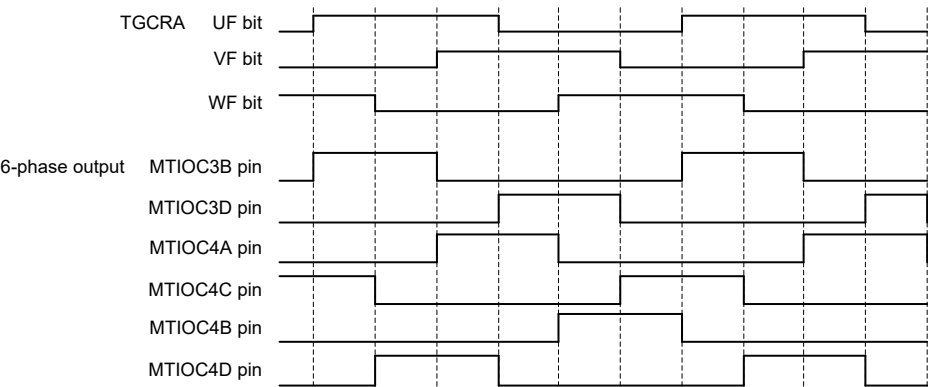
Figure 16.81 Example of Output Phase Switching through UF, VF, and WF Bit Settings (1)
