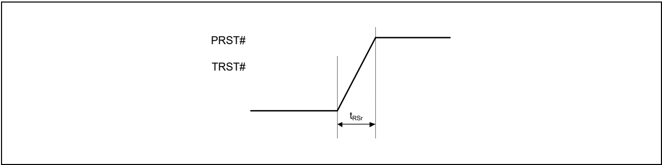
Figure 48.28 Reset Input Timing 2
