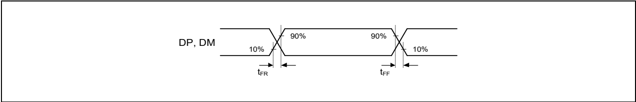
Figure 48.12 USB0_DP, USB1_DP, USB0_DM, and USB1_DM Output Timing (Full-Speed)
