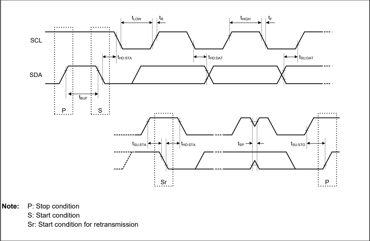
Figure 48.38 Input/Output Timing
