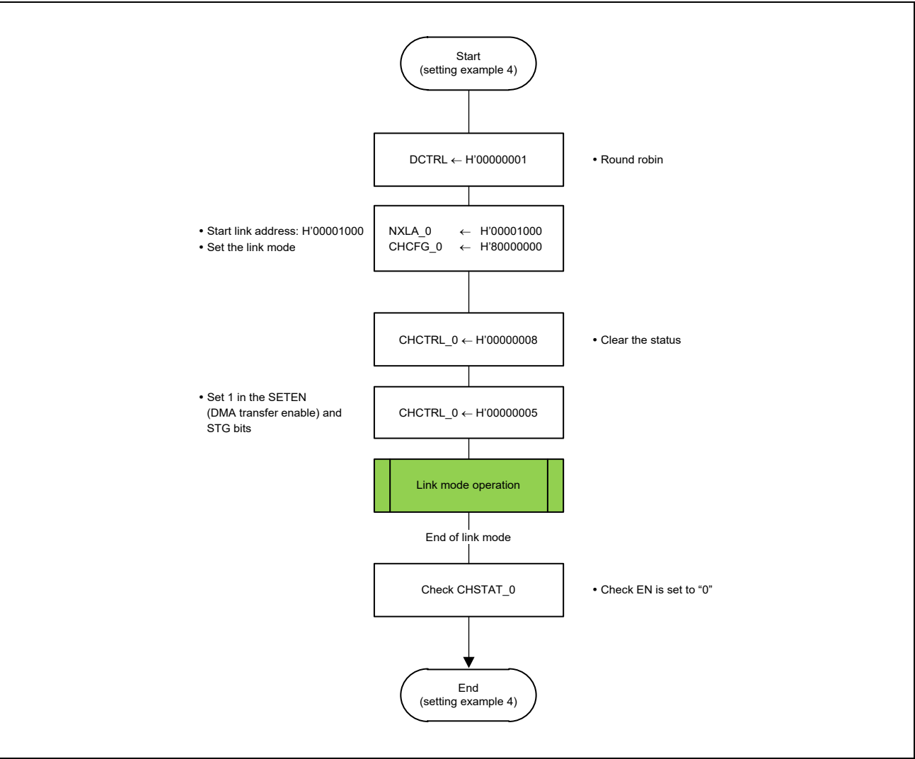
Figure 14.26 Setting Example 4
