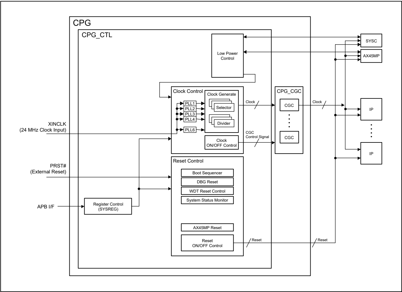
Figure 7.1 CPG Configuration
