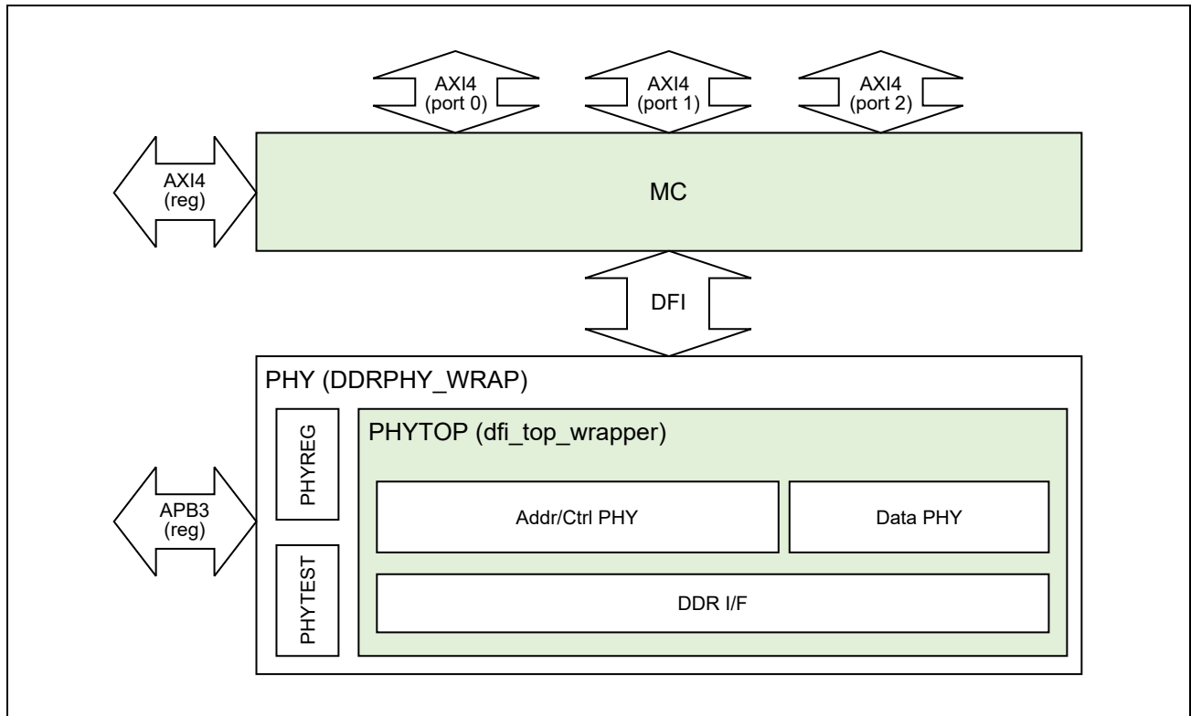
Figure 9.1 Block Diagram
