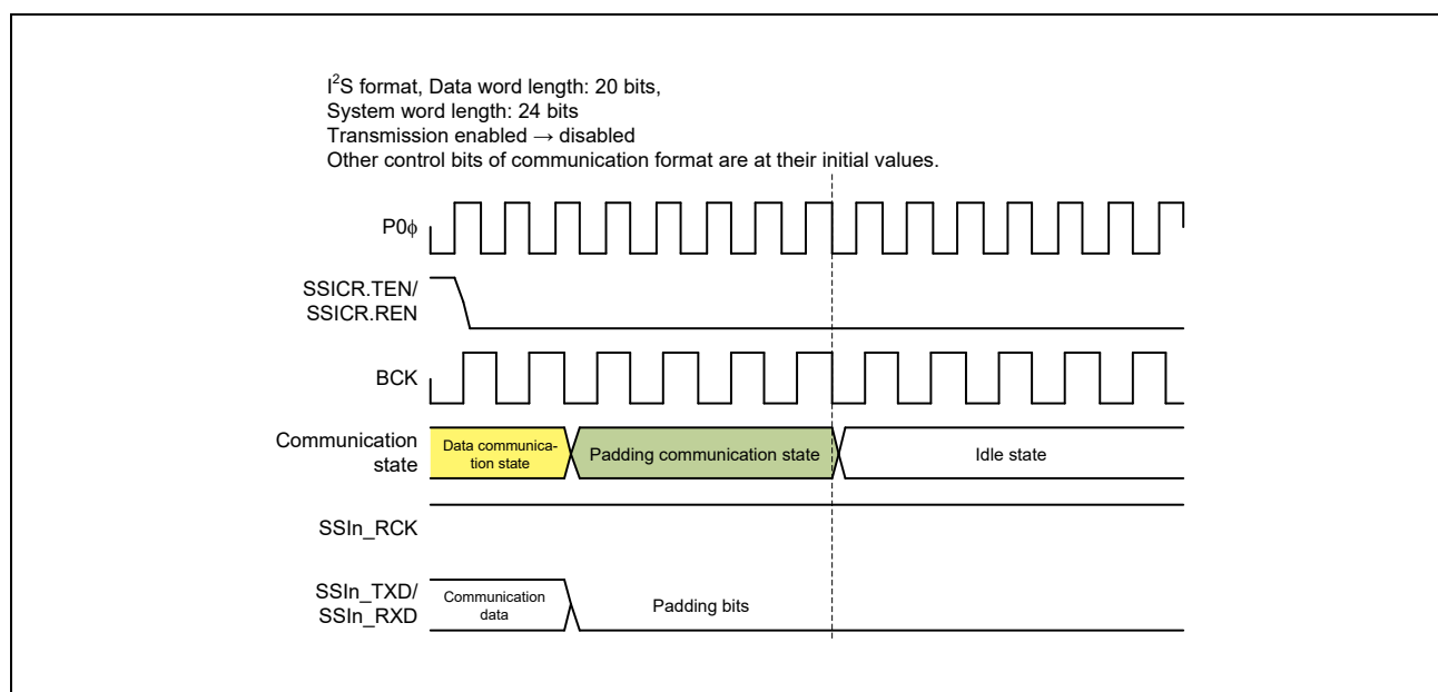
Figure 27.50 Halt from the Padding Communication State
