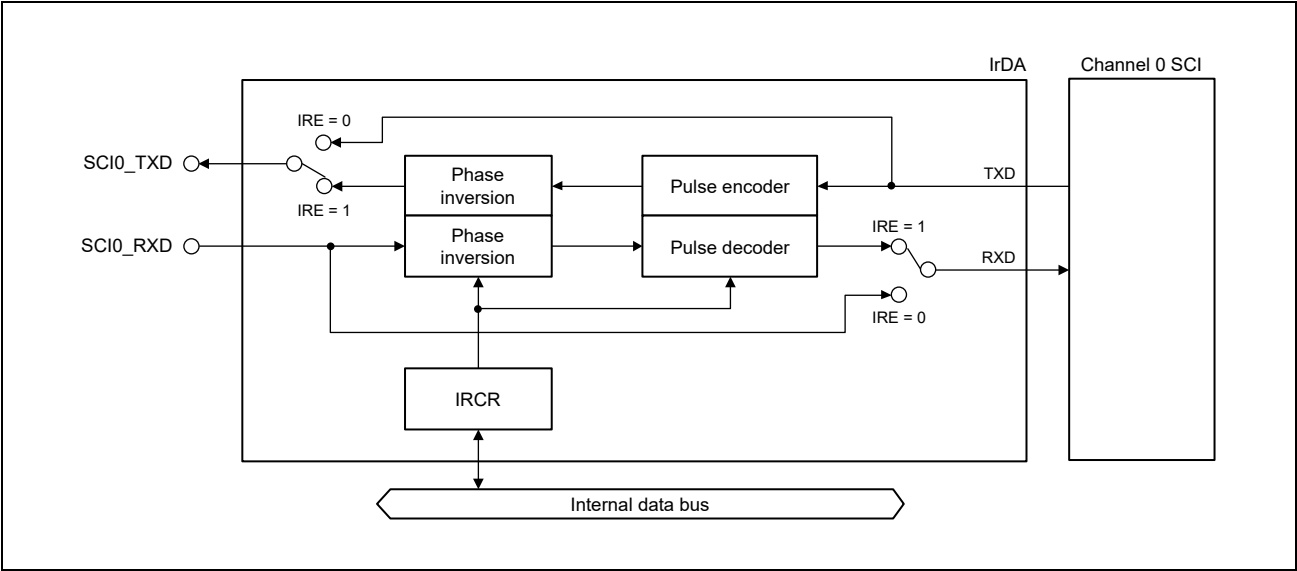
Figure 23.43 Block Diagram
