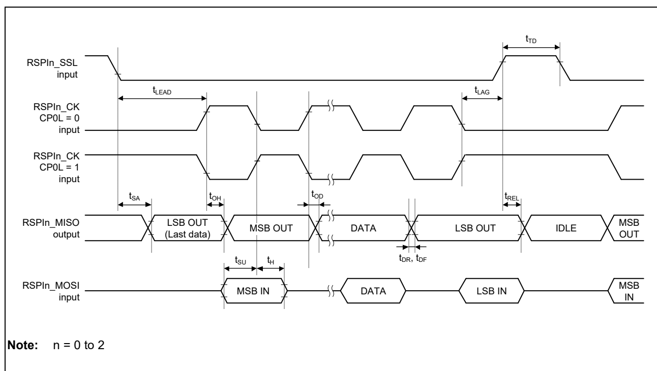
Figure 48.47 Transmission and Reception Timing (Slave, CPHA = 1)
