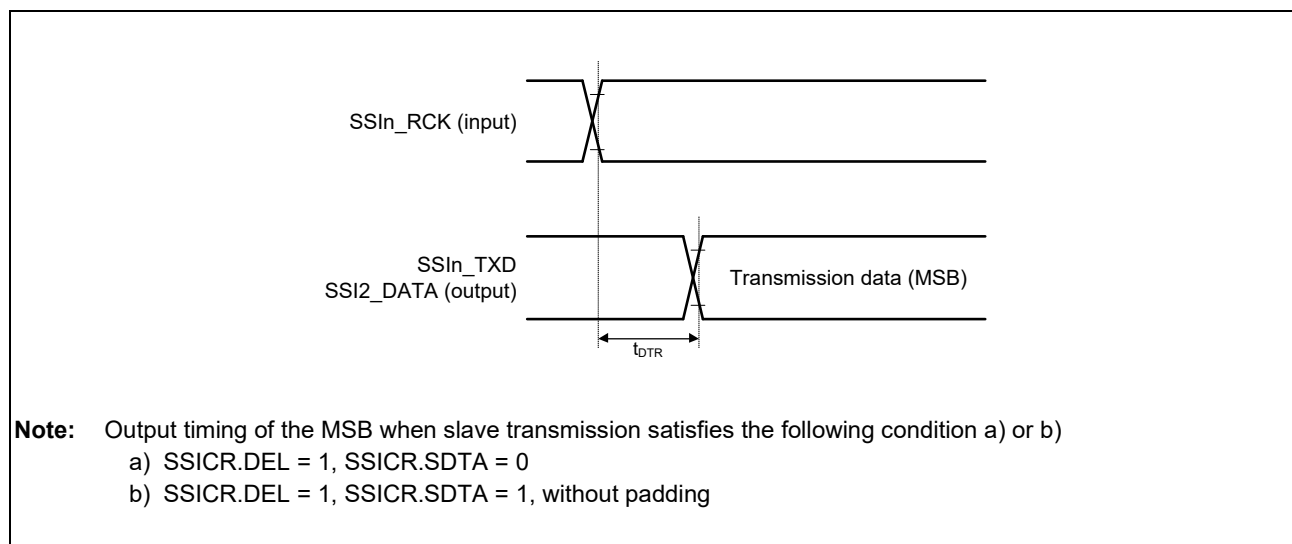
Figure 48.33 Transmission Timing (Slave, in Synchronization with SSILRCK)
