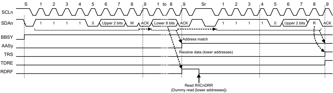
[10-bit address format: Slave transmission]
