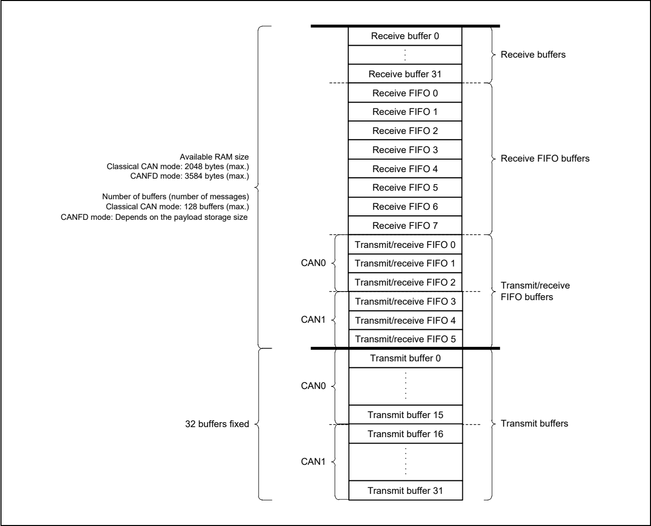
Figure 28.20 Buffer Configuration
