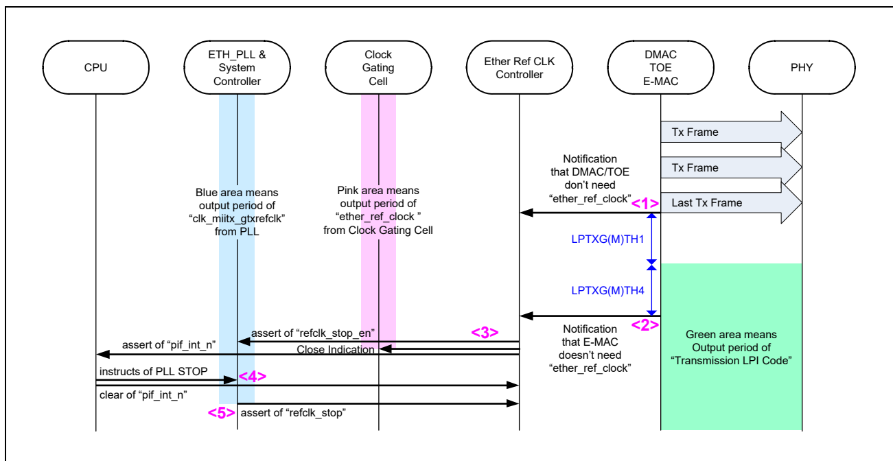
Figure 30.43 Sequence of stopping “clk_miitx_gtx_refclk”
