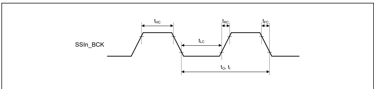
Figure 48.30 Bit Clock Input/Output Timing
