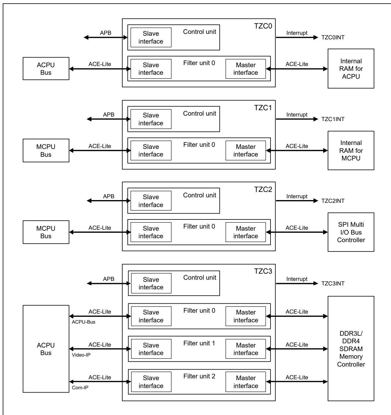
Figure 13.1 Block Diagram
