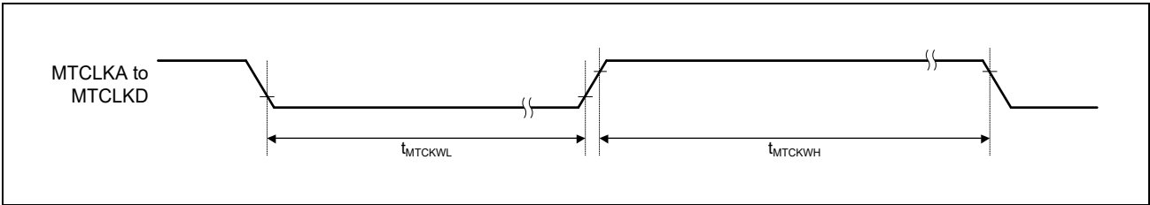
Figure 48.36 MTU3a Clock Input Timing
