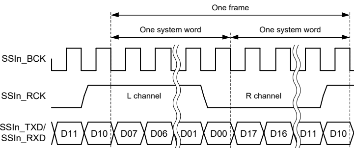
Figure 27.5 LRCK/FS Polarity Setting
