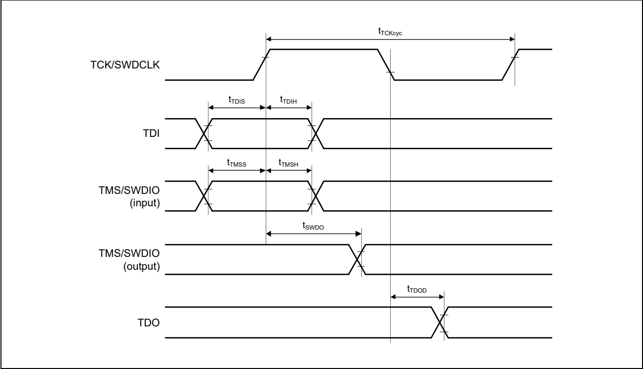
Figure 48.21 Data Transfer Timing
