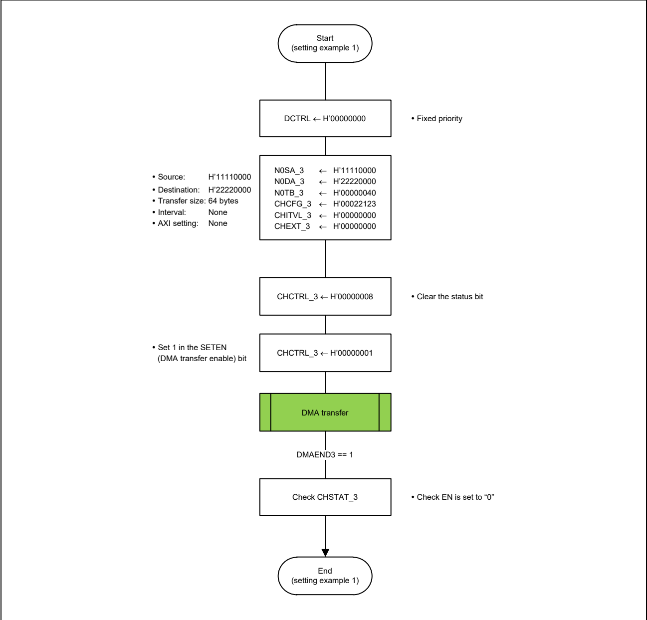
Figure 14.23 Setting Example 1
