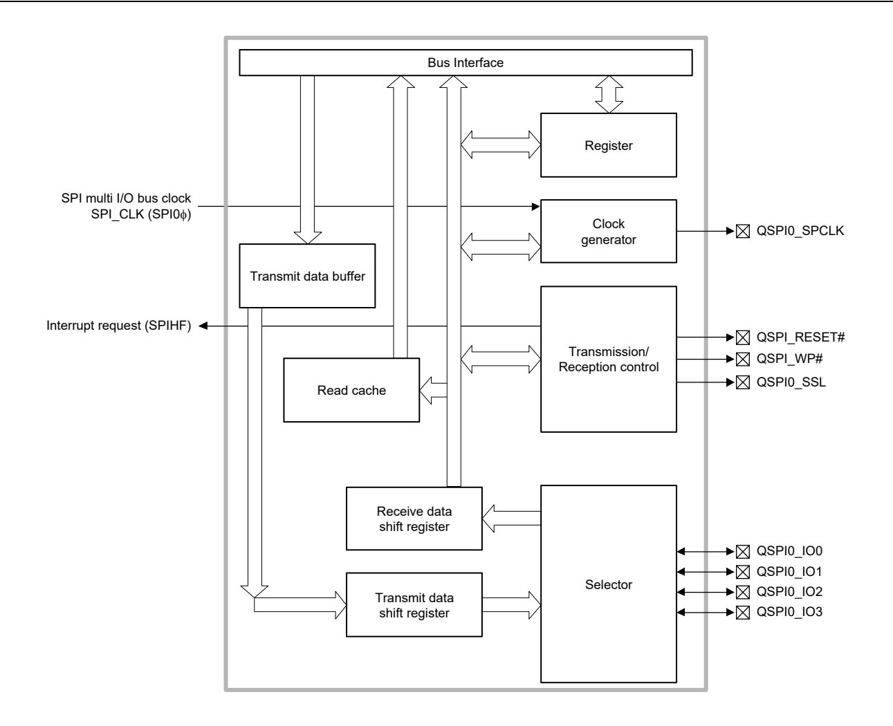
Figure 25.1 Block Diagram
