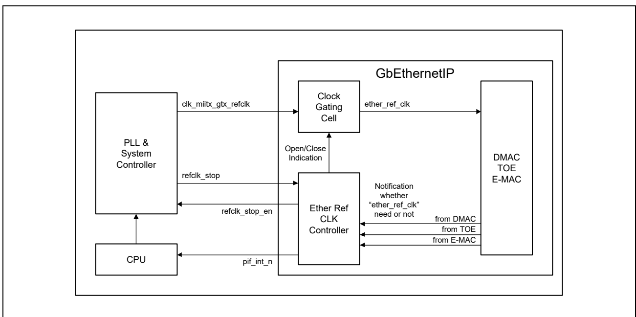
Figure 30.42 Block Diagram
