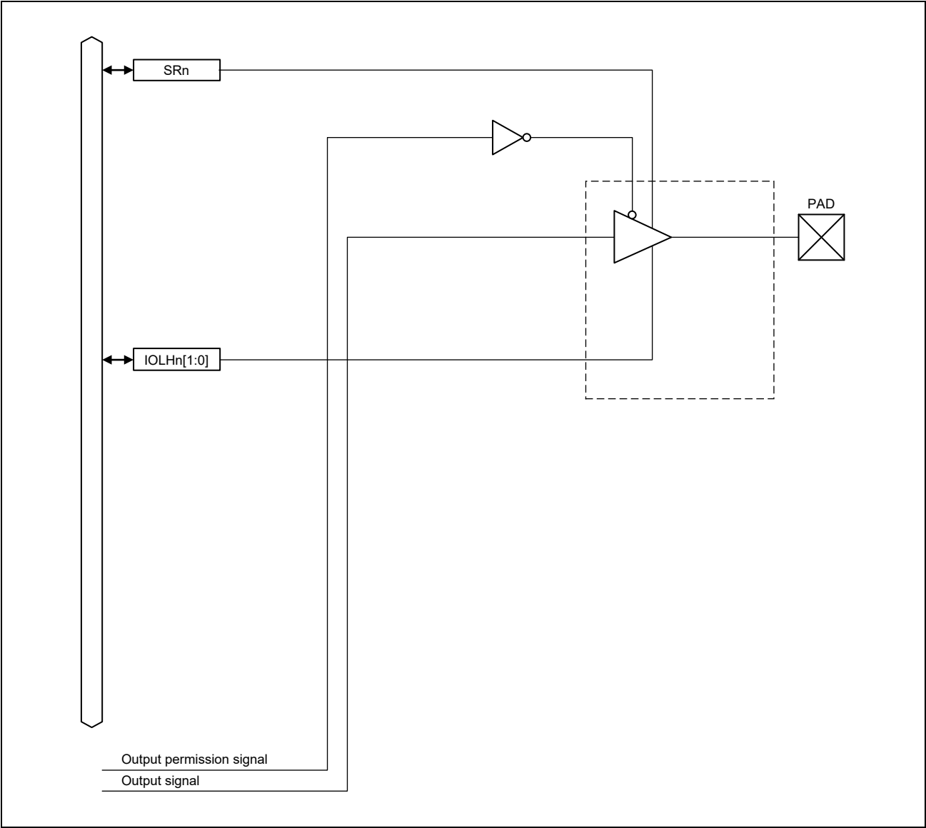
Figure 41.12 TDO
