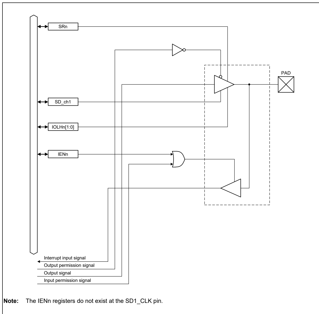
Figure 41.7 SDHI ch1 (SD1_CLK, SD1_CMD, SD1_DATA[3:0])
