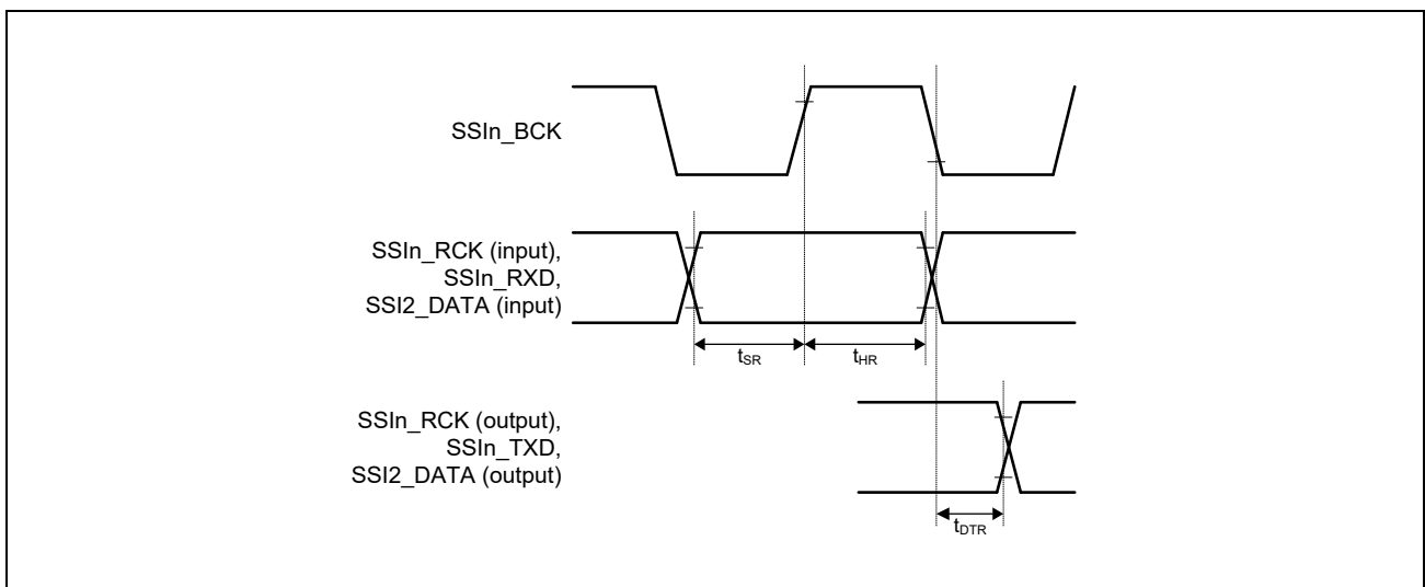
Figure 48.31 Transmission and Reception Timing (SSIBCK Falling Output)
