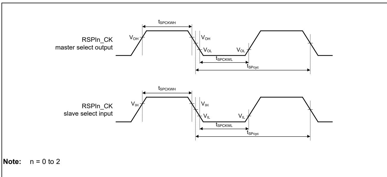
Figure 48.43 Clock Timing
