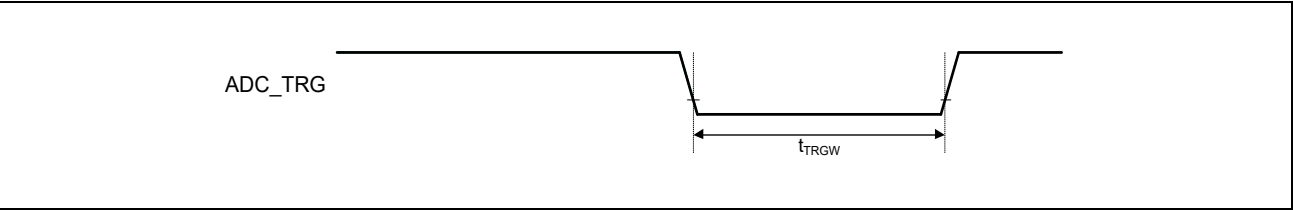
Figure 48.48 ADC Trigger Input Timing
