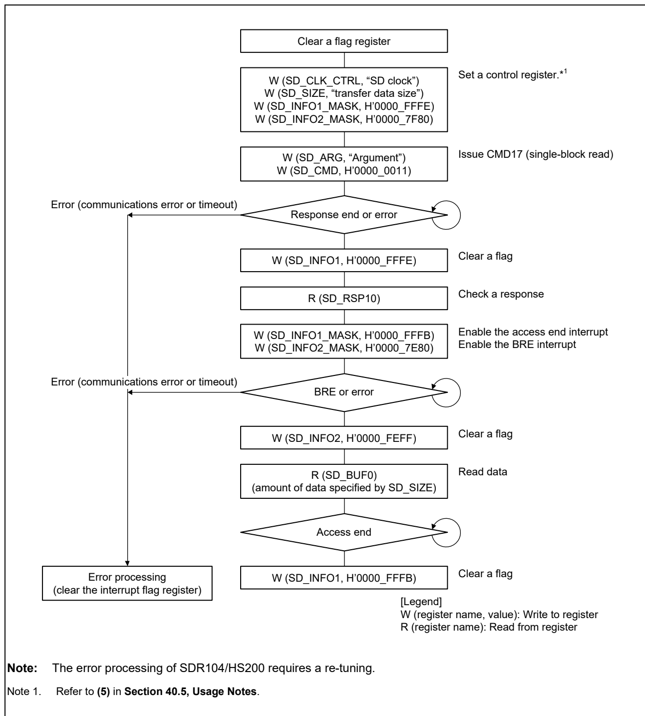
Figure 40.10 Single Block Read Flowchart Example
