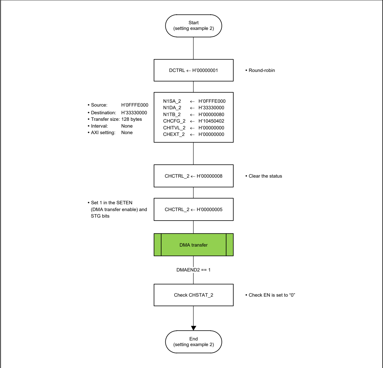
Figure 14.24 Setting Example 2
