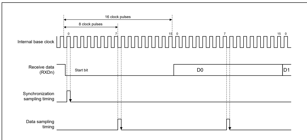
Figure 23.3 Receive Data Sampling Timing in Asynchronous Mode
