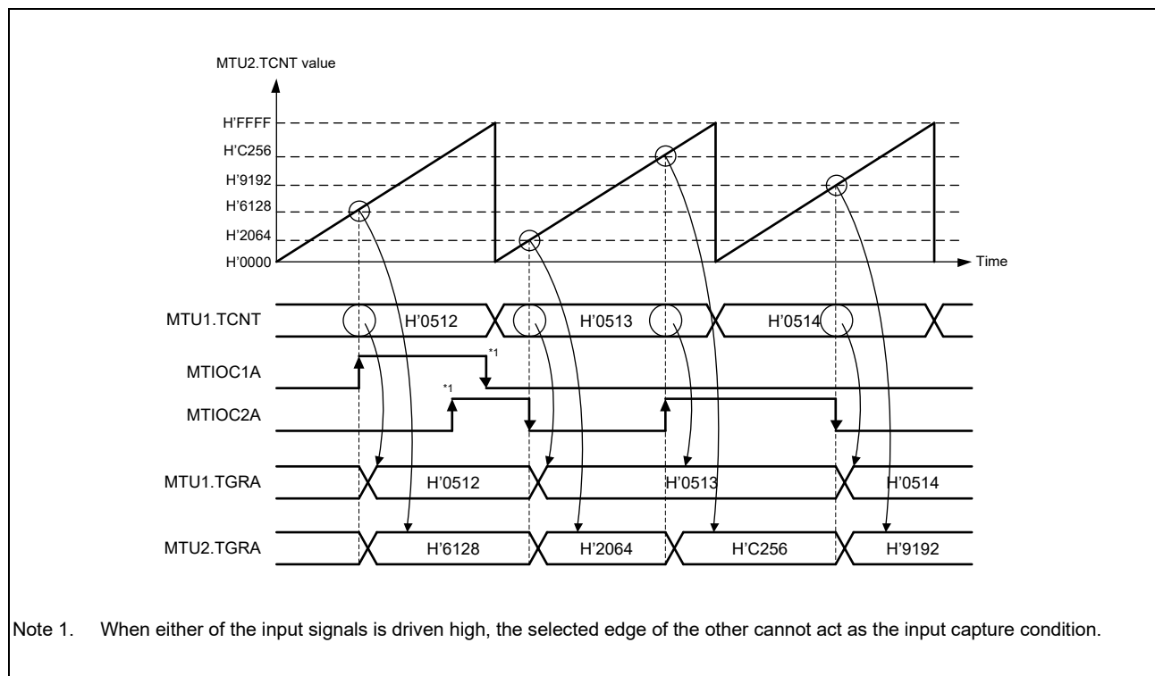
Figure 16.24 Cascaded Operation Example (c)
