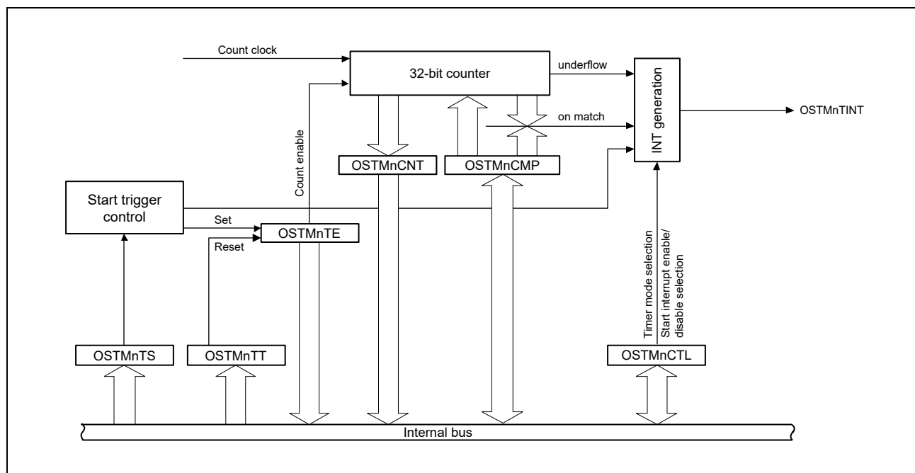
Figure 20.1 Block Diagram of GTM
