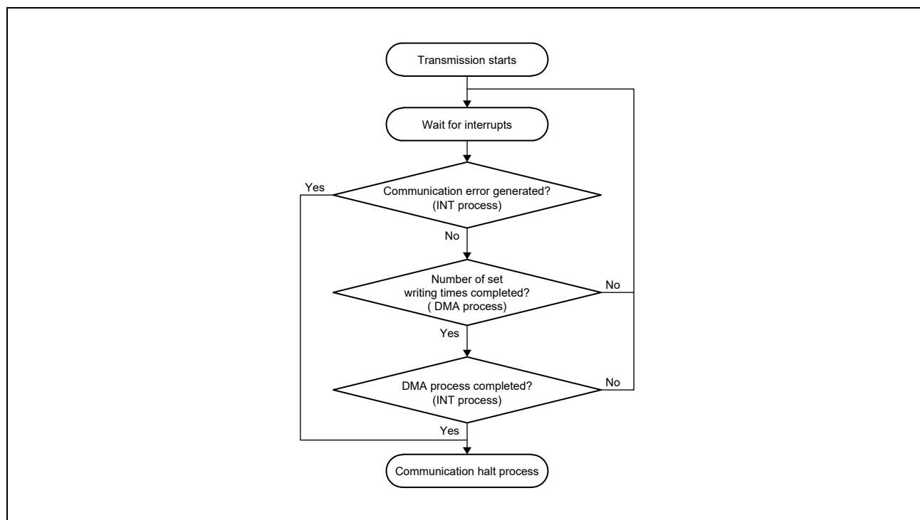
Figure 27.53 Transmission Procedure
