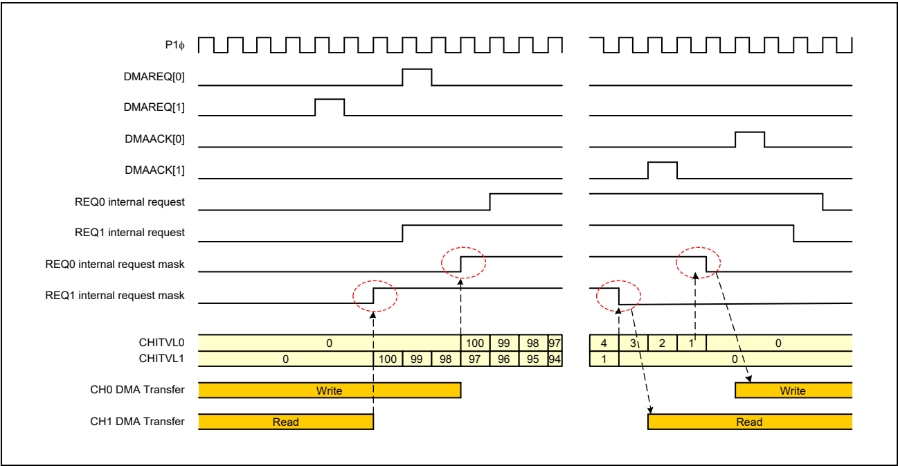
Figure 14.15 Interval Count
