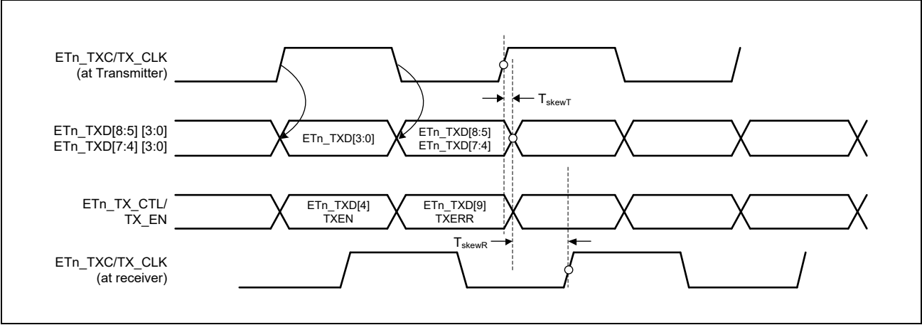
Figure 48.18 Multiplexing & Timing Diagram — RGMII (Transmitter)
