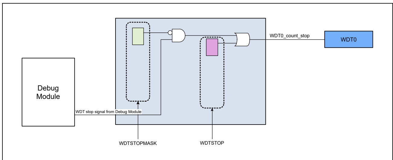
Figure 6.2 Overview of WDT Stop Function
