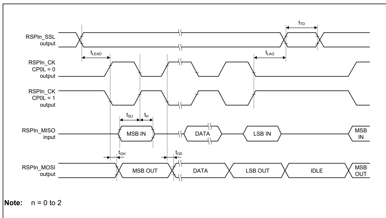
Figure 48.45 Transmission and Reception Timing (Master, CPHA = 1)
