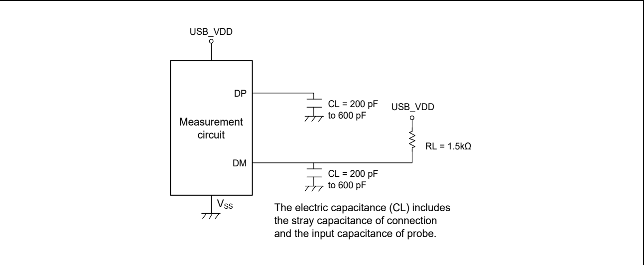
Figure 48.11 Measurement Circuit (Low-Speed)
