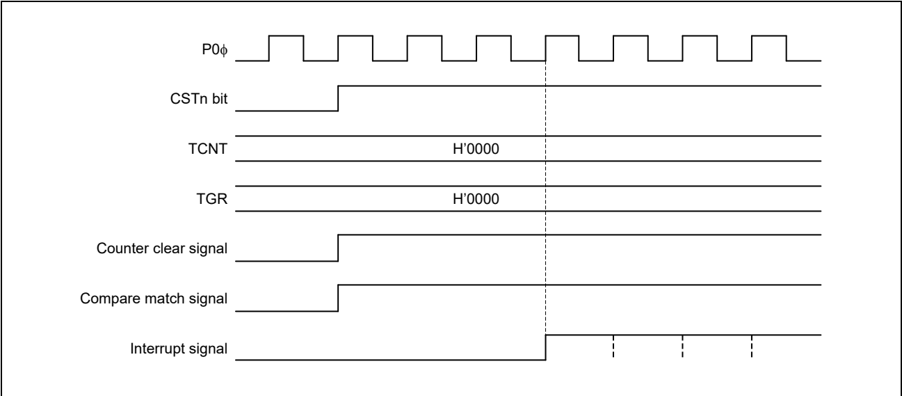
Figure 16.151 Continuous Output of Interrupt Signal in Response to a Compare Match
