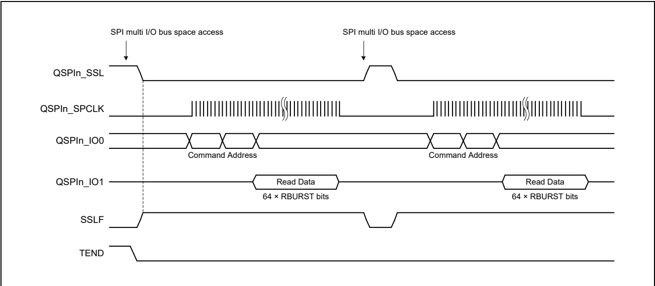
Figure 25.8 Burst Read Timing for Non-Continuous Address (SSLE Bit = 1)
