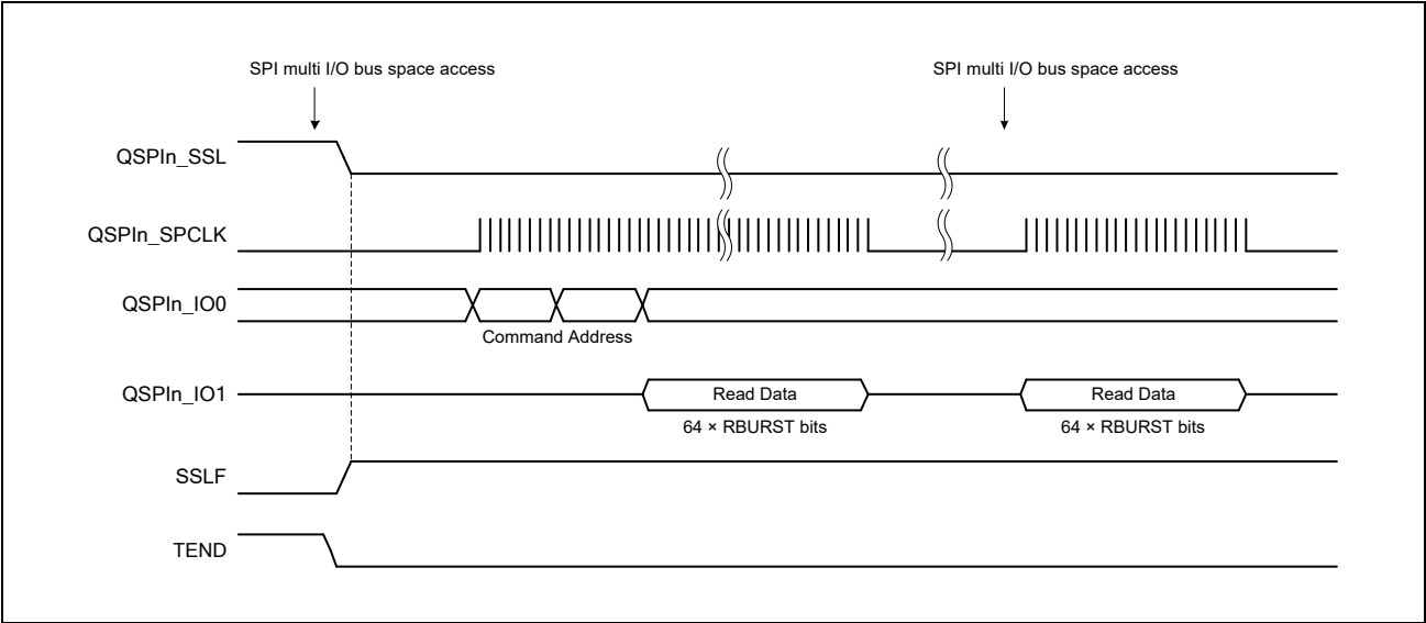
Figure 25.7 Burst Read Timing for Continuous Address (SSLE Bit = 1)
