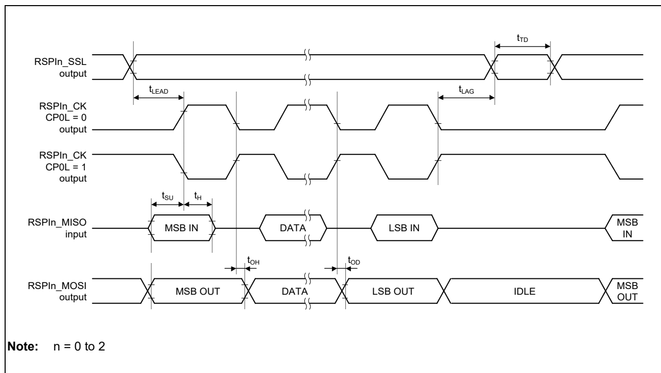
Figure 48.44 Transmission and Reception Timing (Master, CPHA = 0)
