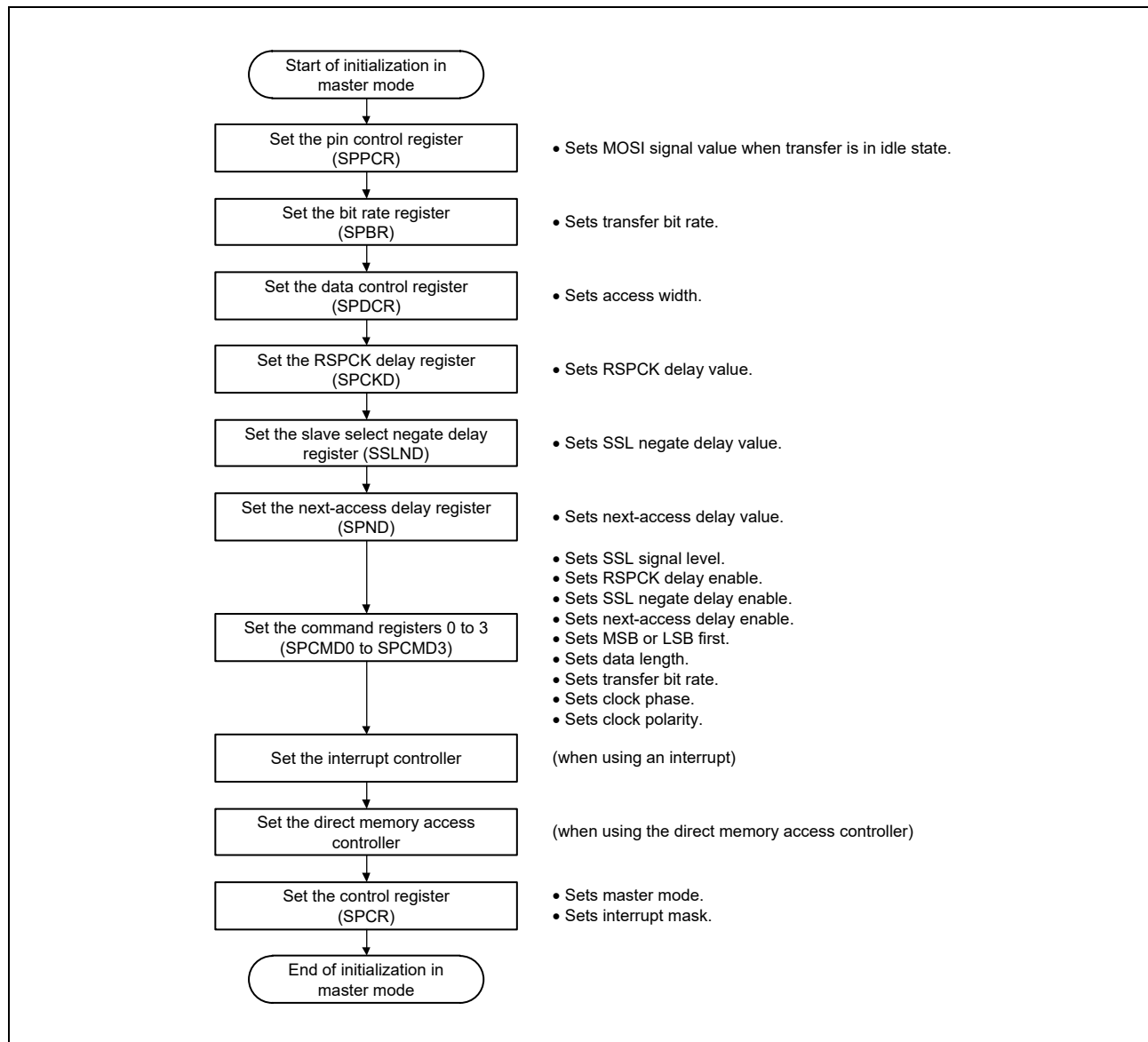
Figure 24.17 Example of Initialization Flowchart in Master Mode
