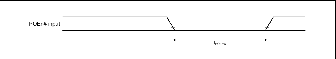
Figure 48.37 POEn# Input Pulse Timing
