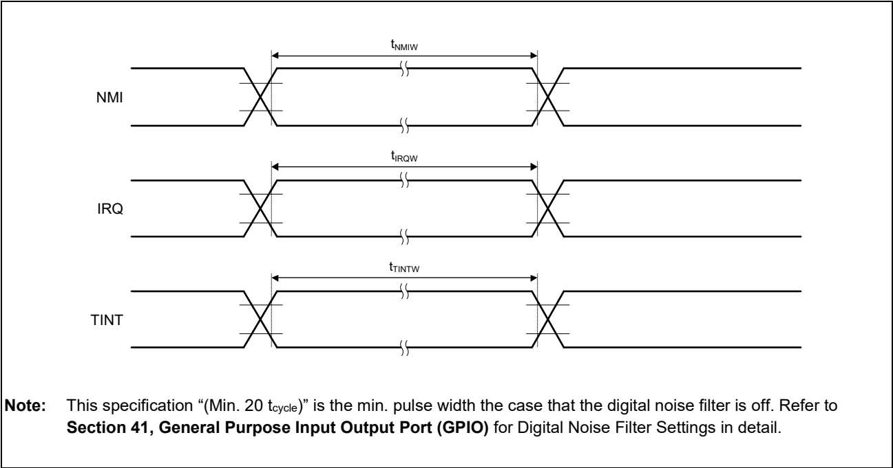
Figure 48.29 Interrupt Signal Input Timing
