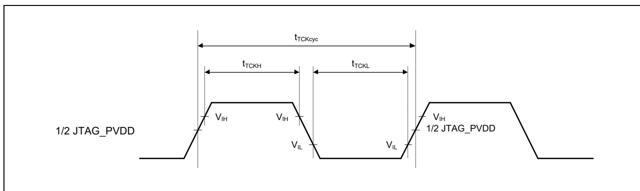
Figure 48.20 TCK_SWCLK Input Timing
