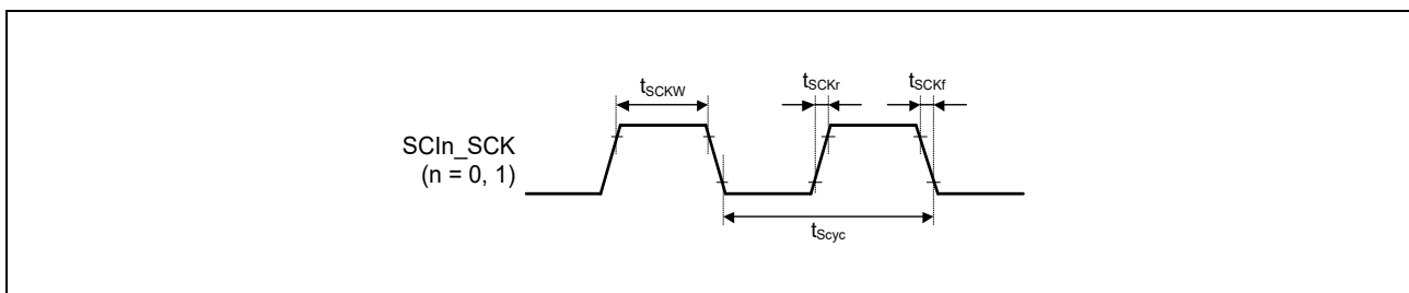
Figure 48.41 SCK Input Clock Timing
