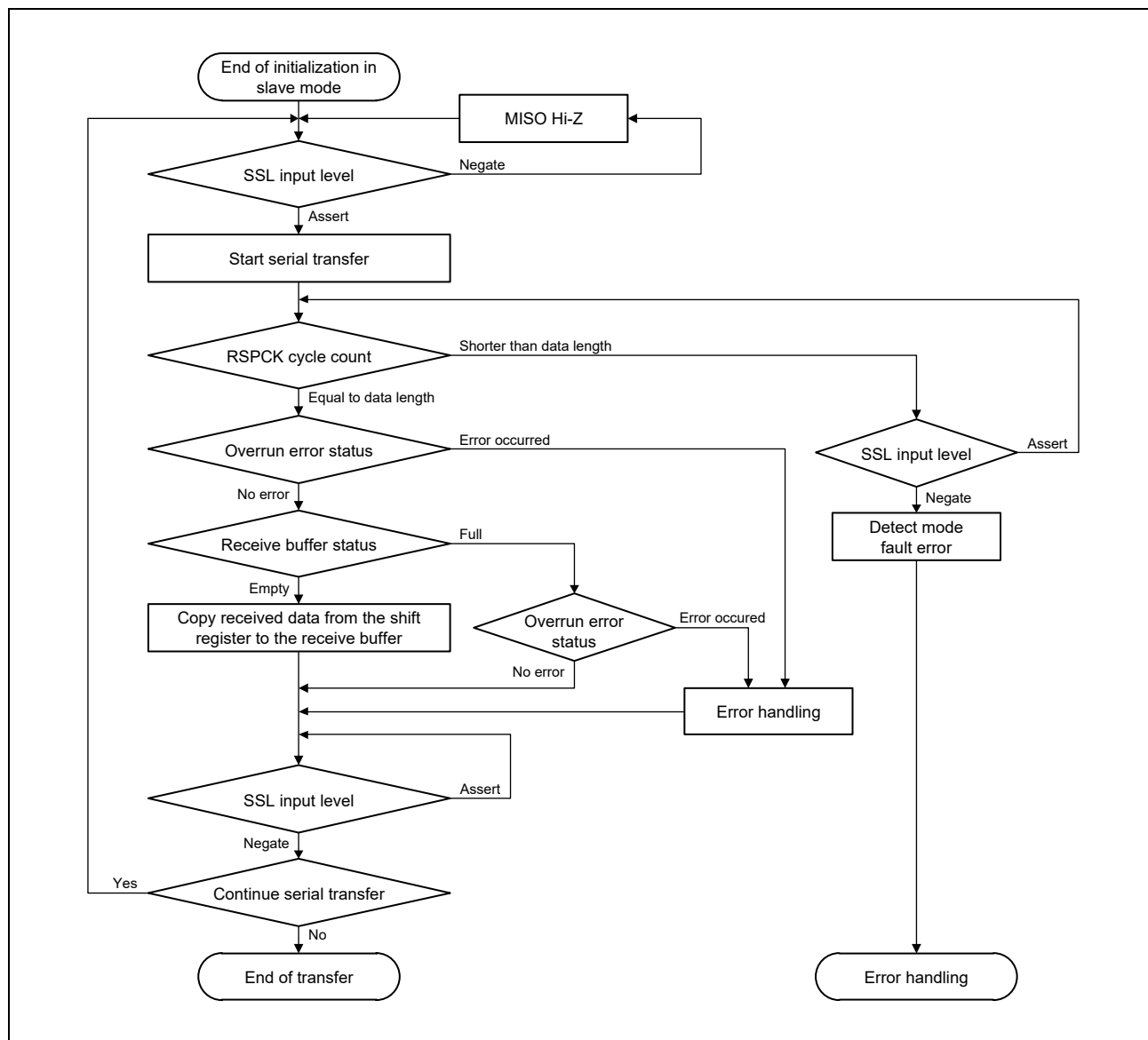
Figure 24.20 Transfer Operation Flowchart in Slave (CPHA = 0)
