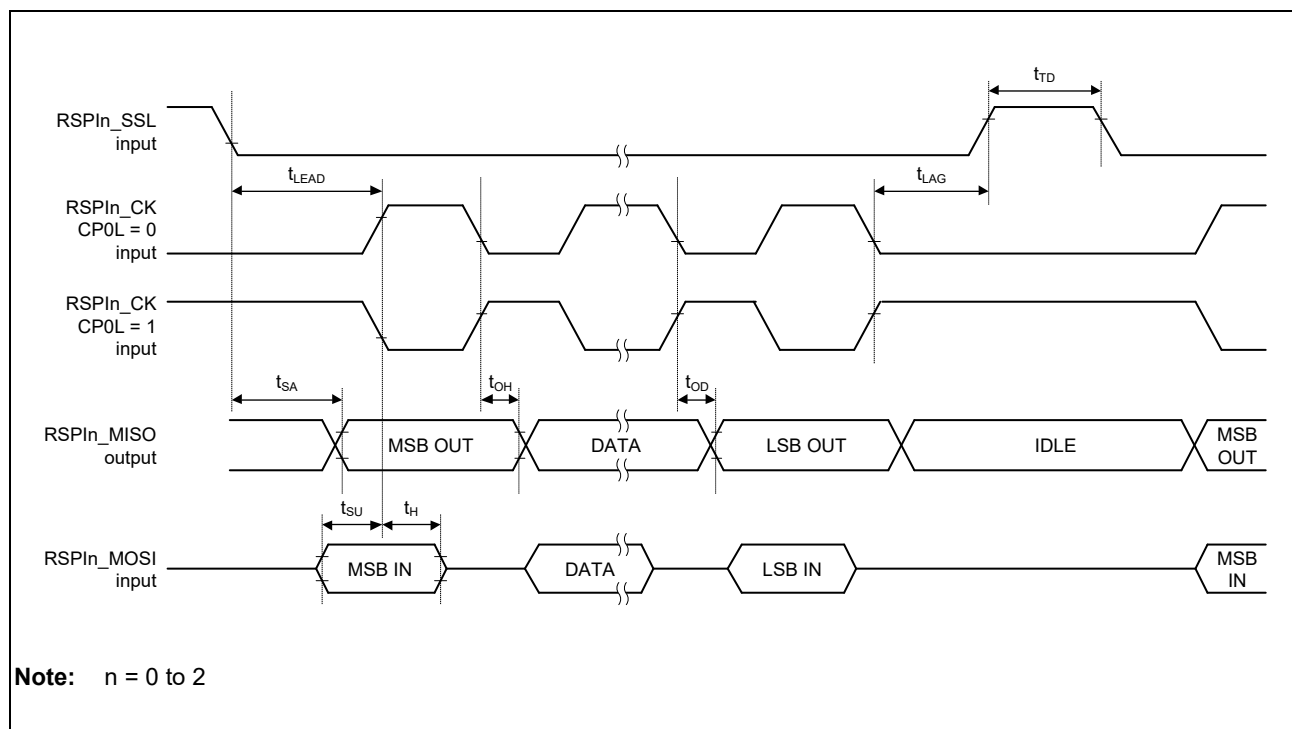
Figure 48.46 Transmission and Reception Timing (Slave, CPHA = 0)
