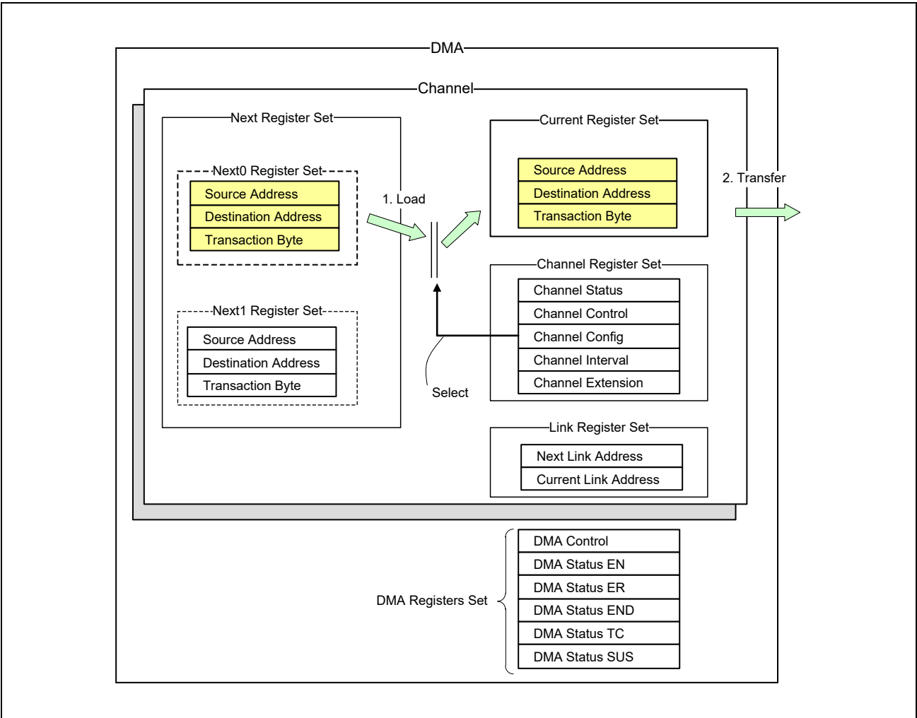
Figure 14.1 Register Configuration
