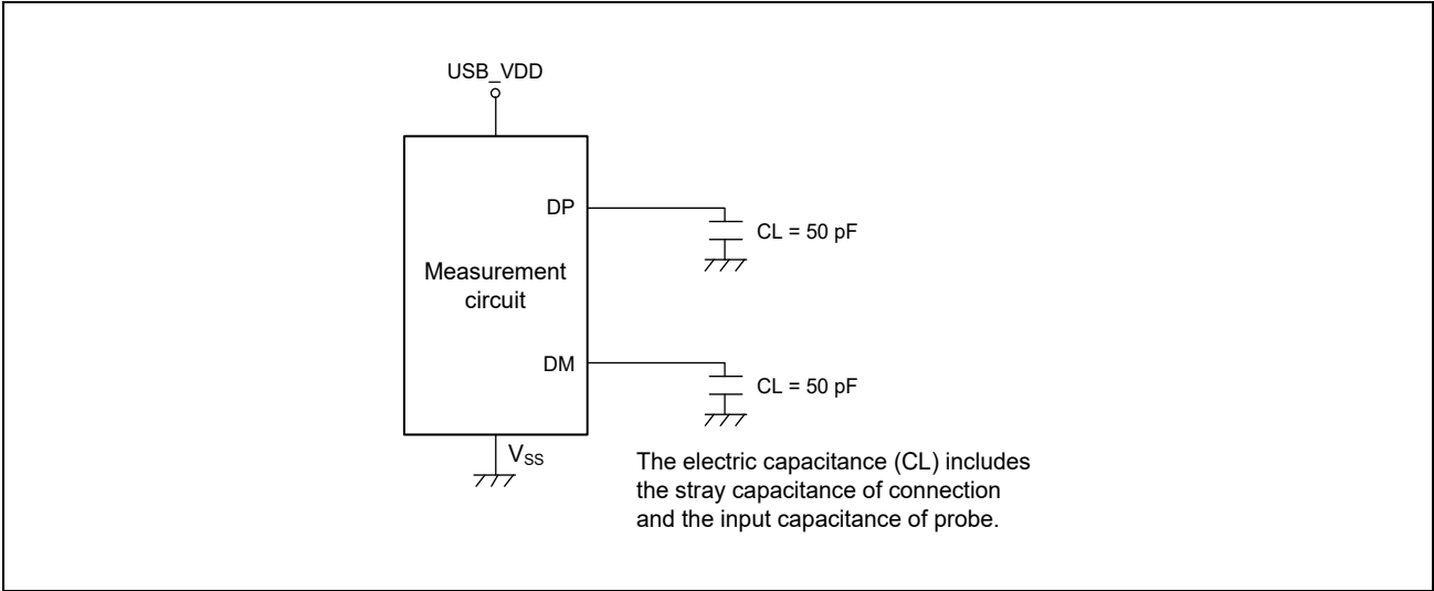
Figure 48.13 Measurement Circuit (Full-Speed)
