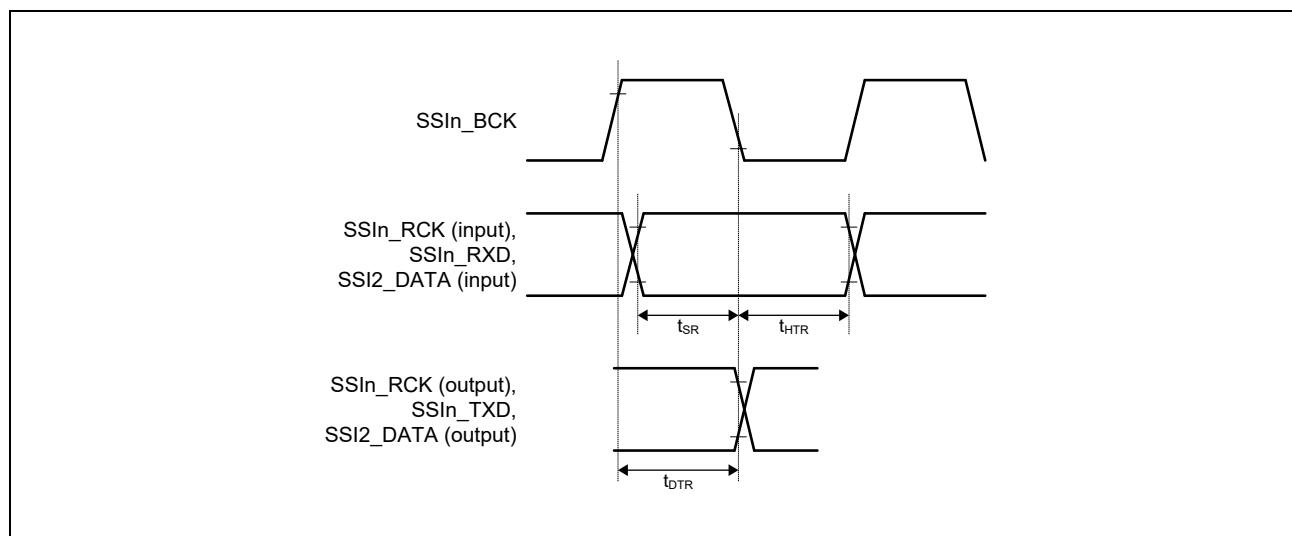
Figure 48.32 Transmission and Reception Timing (SSIBCK Rising Output)
