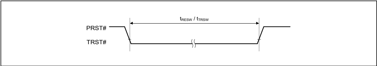
Figure 48.27 Reset Input Timing 1
