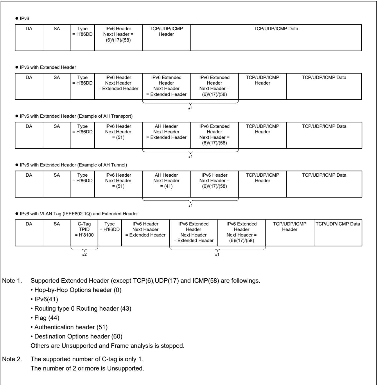
Figure 30.32 Supported Frame Format of IPv6
