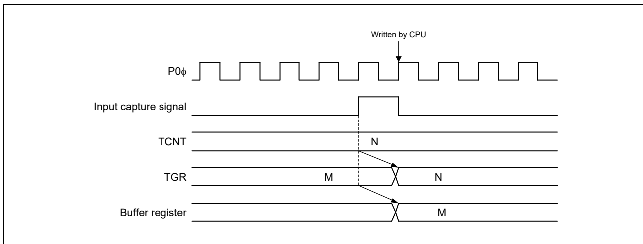
Figure 16.142 Contention between Buffer Register Write Operation and Input Capture
