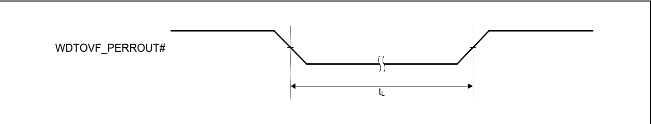
Figure 48.49 Watchdog Timer Output Timing
