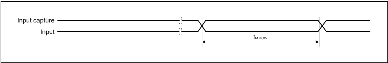
Figure 48.35 MTU3a Input Capture Input Timing
