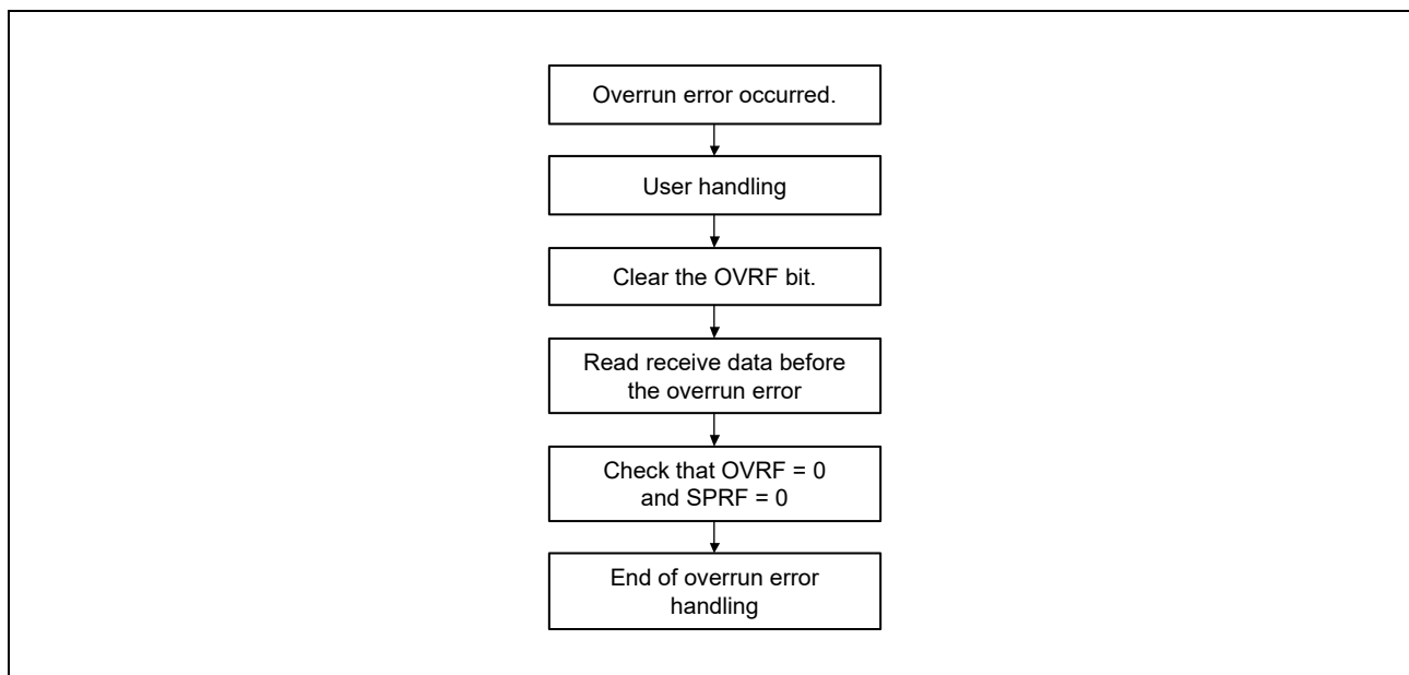
Figure 24.22 Error Handling (Overrun Error)
