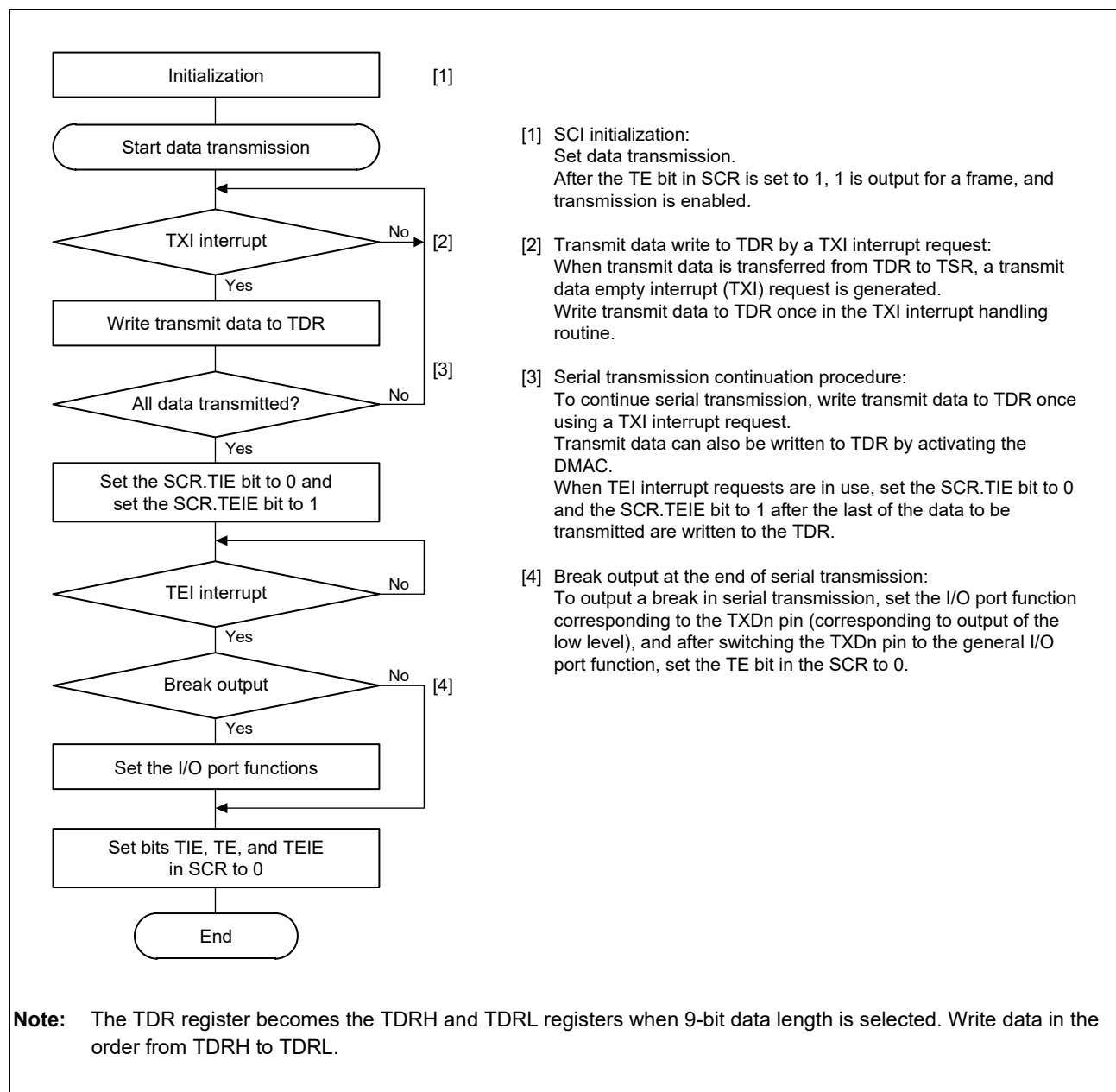
Figure 23.9 Example of Serial Transmission Flowchart in Asynchronous Mode
