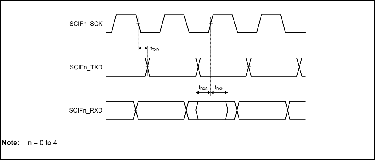
Figure 48.40 SCIFA Input/Output Timing in Clocked Synchronous Mode
