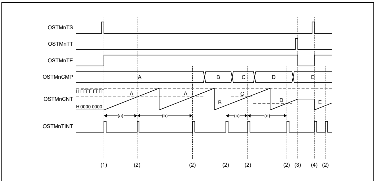
Figure 20.6 Timing Diagram of OSTM in Free-Run Compare Mode
