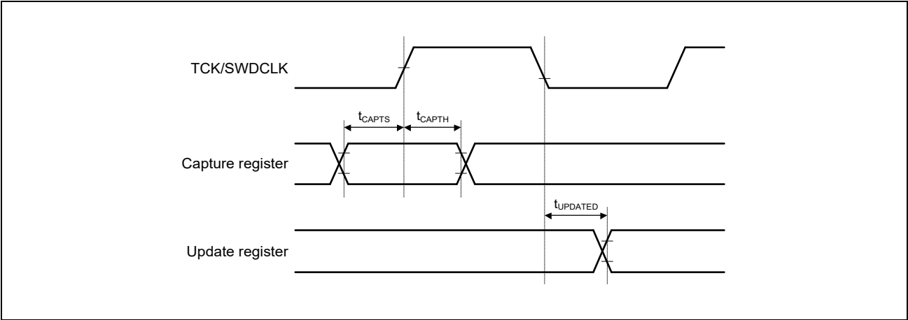
Figure 48.22 Boundary Scan Input/Output I/O Timing
