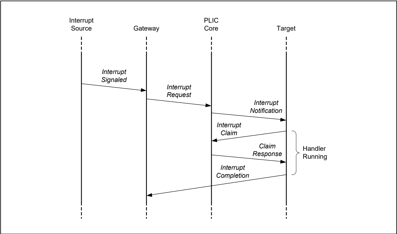
Figure 8.2 Interrupt Flow for Level Interrupt
