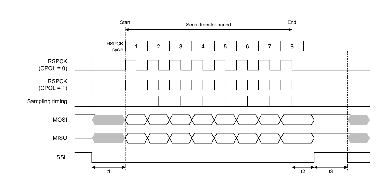
Figure 24.7 Transfer Format (CPHA = 1)
