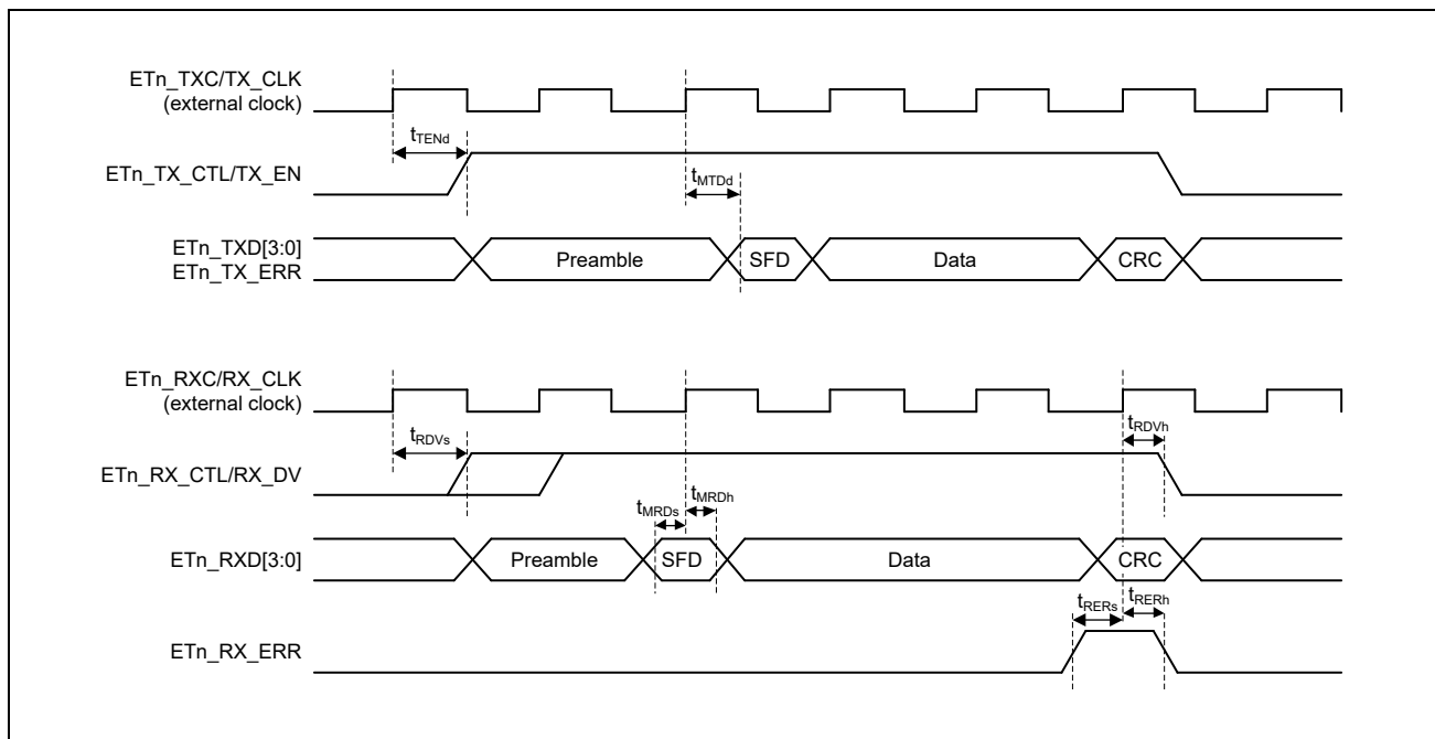
Figure 48.17 MII Transmission Timing
