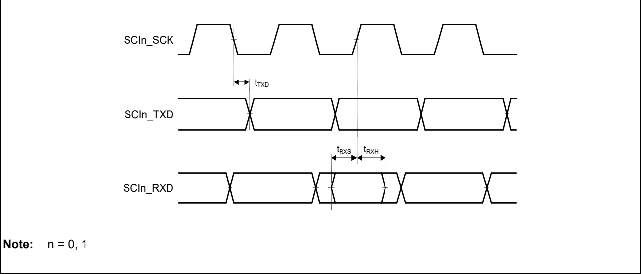
Figure 48.42 SCIFA Input/Output Timing in Clocked Synchronous Mode
