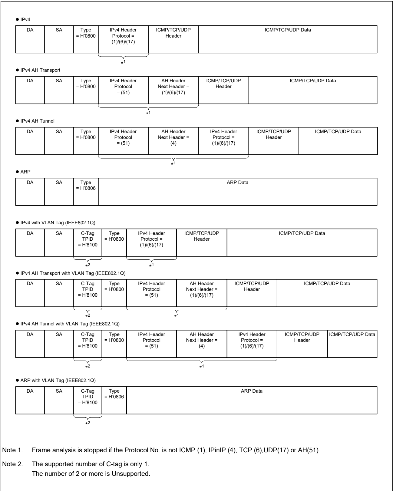
Figure 30.31 Supported Frame of IPv4
