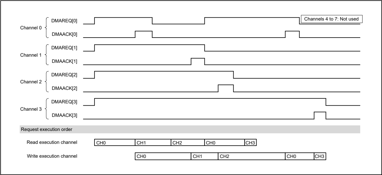
Figure 14.13 Fixed Priority Mode (Number of Channels = 4, REQD = 1)
