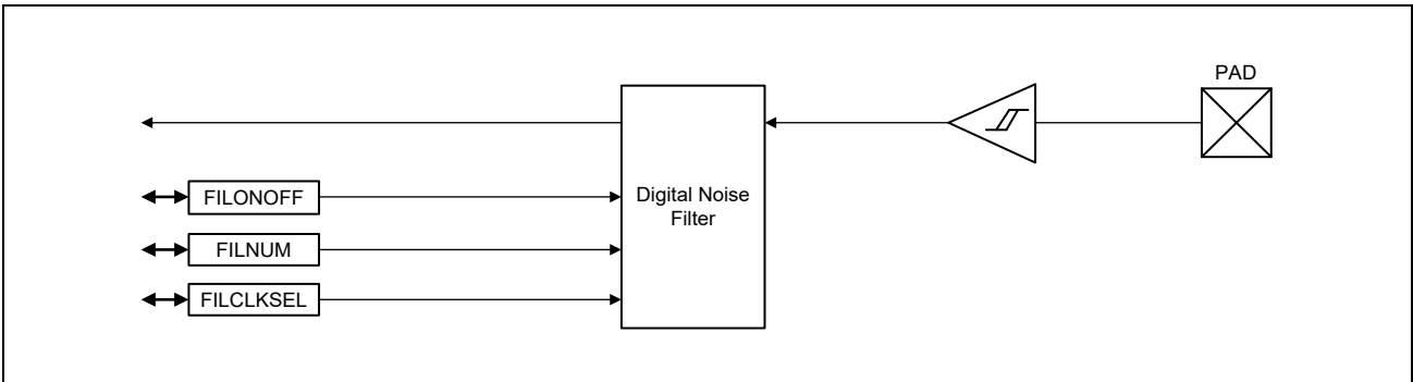
Figure 41.10 NMI
