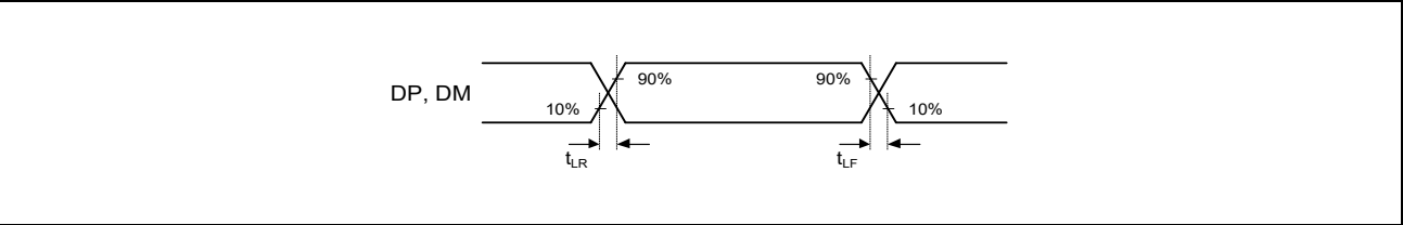
Figure 48.10 USB0_DP, USB1_DP, USB0_DM, and USB1_DM Output Timing (Low-Speed)
