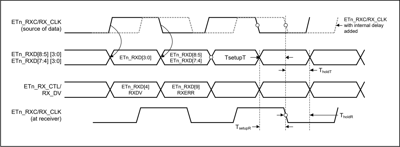
Figure 48.19 Multiplexing & Timing Diagram — RGMII-ID (Receiver)
